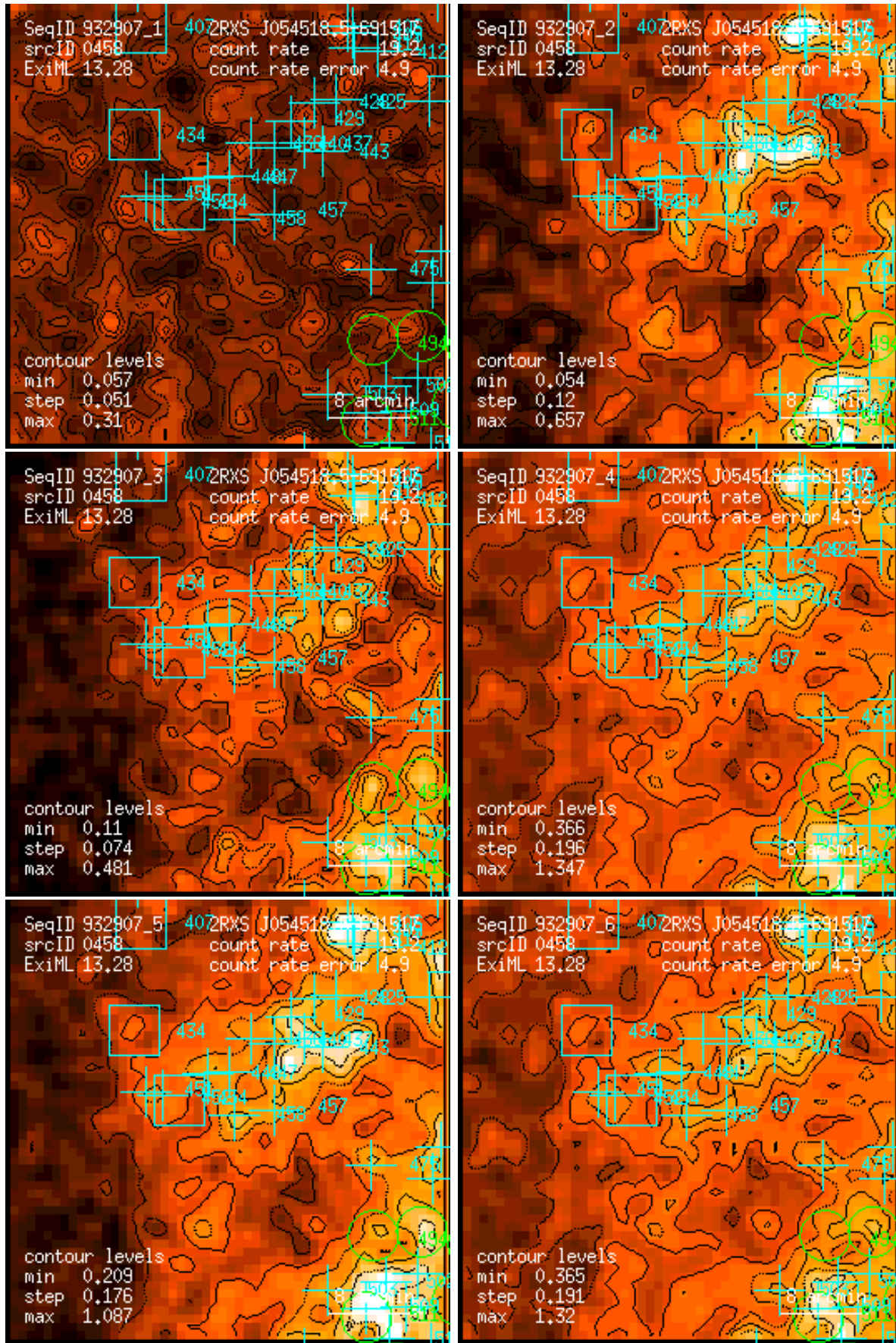
Figure 458: RASS 932907: detection 0458: band rate images, Gaussian filter: (1) PSPC channels 11 – 41, (2) 52 – 90, (3) 91 – 201, (4) 11 – 235, (5) 52 – 201, (6) 11 – 201. Broad band rates in counts/ks. Band rate contour levels in counts/ks/arcmin 2 .
