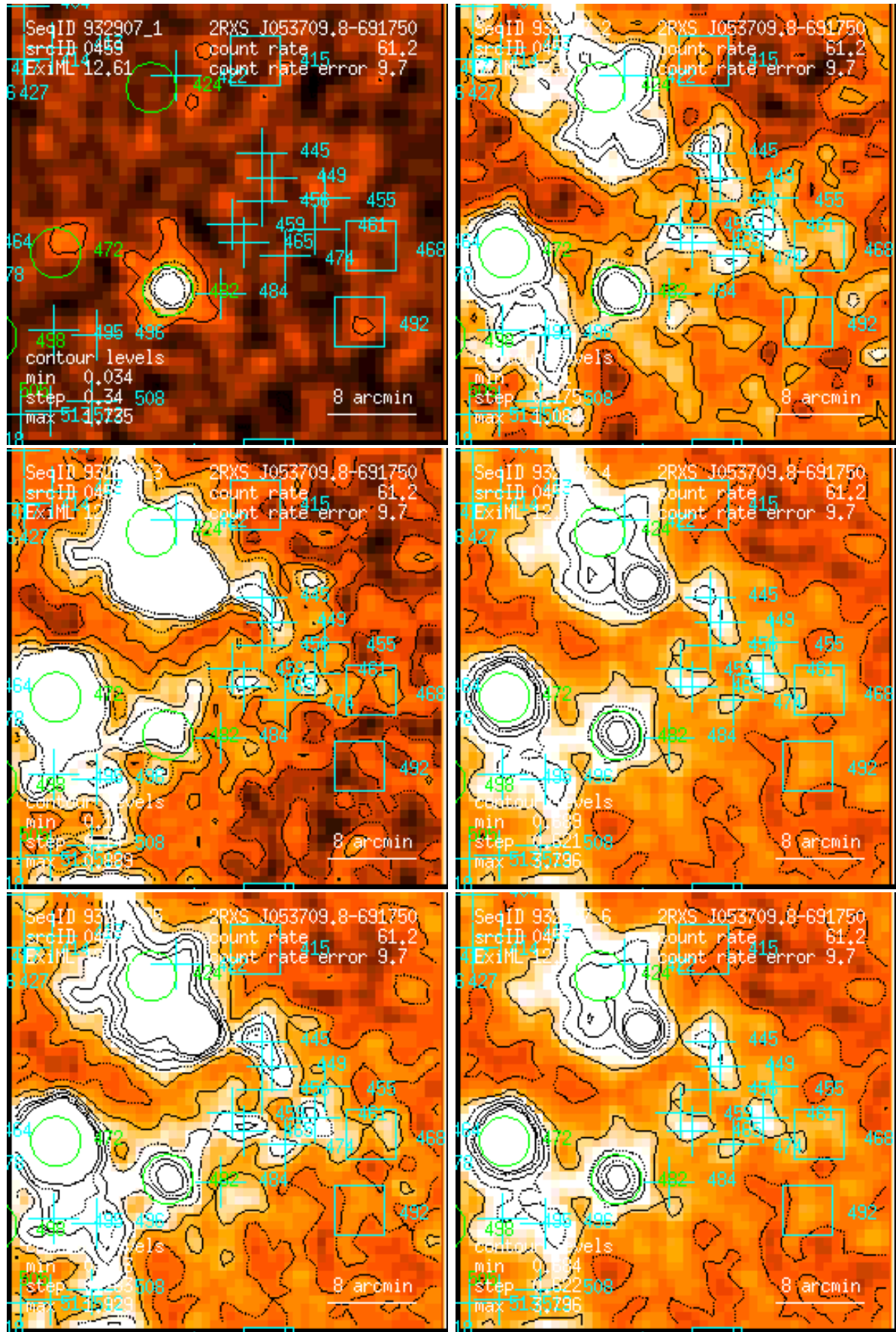
Figure 459: RASS 932907: detection 0459: band rate images, Gaussian filter: (1) PSPC channels 11 – 41, (2) 52 – 90, (3) 91 – 201, (4) 11 – 235, (5) 52 – 201, (6) 11 – 201. Broad band rates in counts/ks. Band rate contour levels in counts/ks/arcmin 2 .
