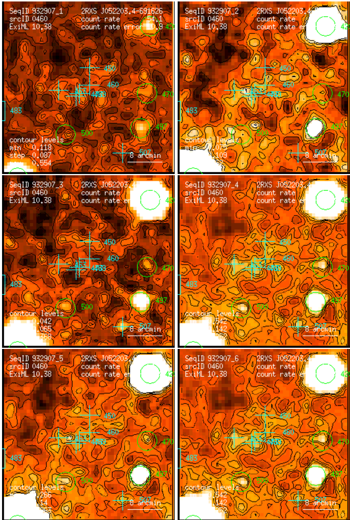
Figure 460: RASS 932907: detection 0460: band rate images, Gaussian filter: (1) PSPC channels 11 – 41, (2) 52 – 90, (3) 91 – 201, (4) 11 – 235, (5) 52 – 201, (6) 11 – 201. Broad band rates in counts/ks. Band rate contour levels in counts/ks/arcmin 2 .
