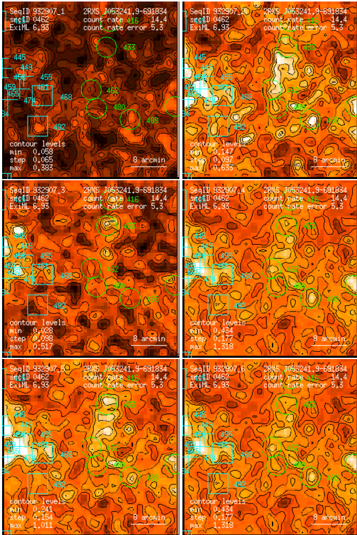
Figure 462: RASS 932907: detection 0462: band rate images, Gaussian filter: (1) PSPC channels 11 – 41, (2) 52 – 90, (3) 91 – 201, (4) 11 – 235, (5) 52 – 201, (6) 11 – 201. Broad band rates in counts/ks. Band rate contour levels in counts/ks/arcmin 2 .
