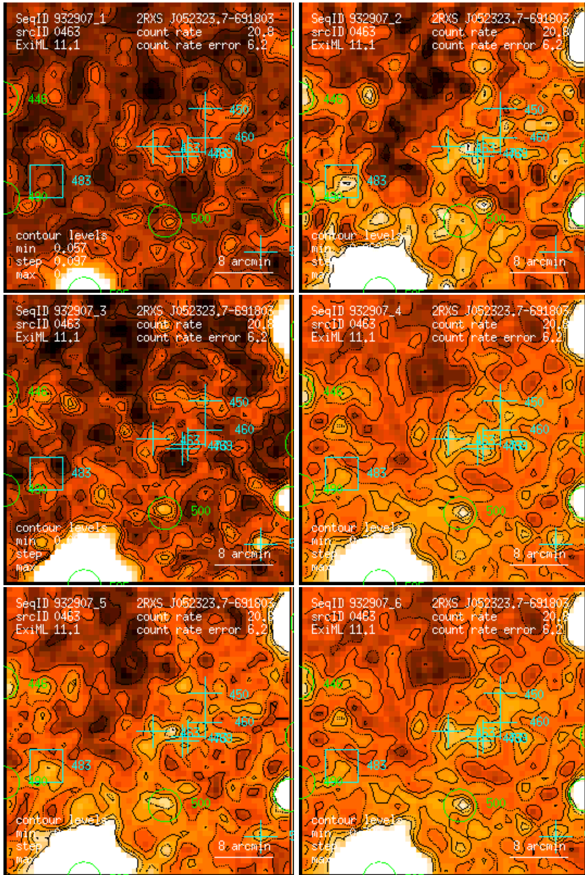
Figure 463: RASS 932907: detection 0463: band rate images, Gaussian filter: (1) PSPC channels 11 – 41, (2) 52 – 90, (3) 91 – 201, (4) 11 – 235, (5) 52 – 201, (6) 11 – 201. Broad band rates in counts/ks. Band rate contour levels in counts/ks/arcmin 2 .
