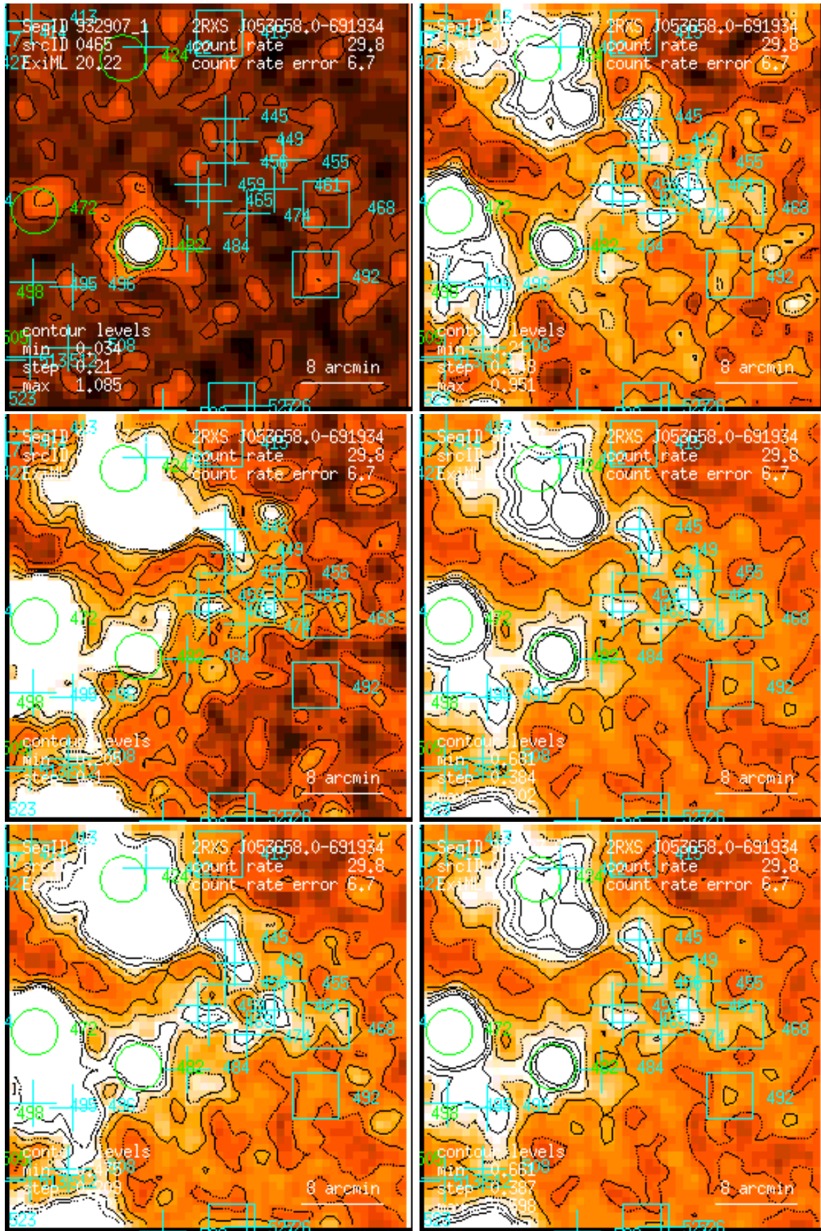
Figure 465: RASS 932907: detection 0465: band rate images, Gaussian filter: (1) PSPC channels 11 – 41, (2) 52 – 90, (3) 91 – 201, (4) 11 – 235, (5) 52 – 201, (6) 11 – 201. Broad band rates in counts/ks. Band rate contour levels in counts/ks/arcmin 2 .
