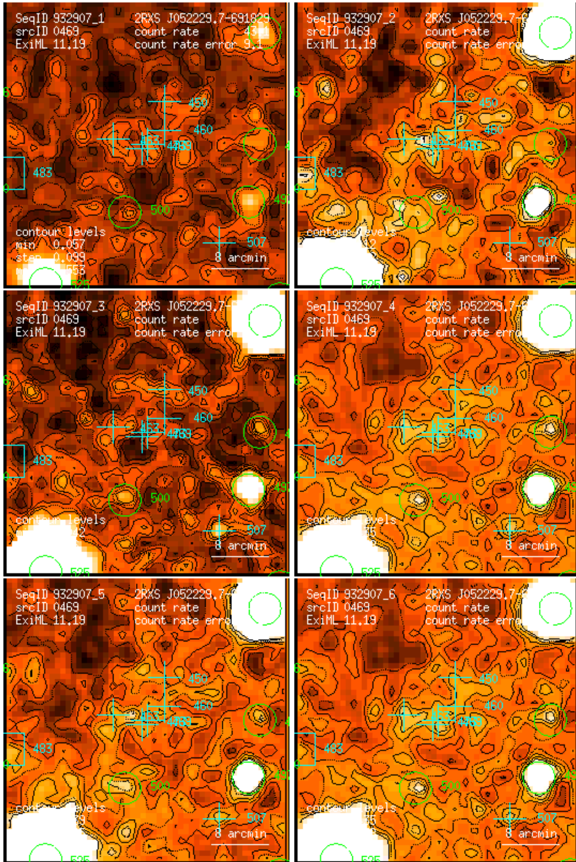
Figure 469: RASS 932907: detection 0469: band rate images, Gaussian filter: (1) PSPC channels 11 – 41, (2) 52 – 90, (3) 91 – 201, (4) 11 – 235, (5) 52 – 201, (6) 11 – 201. Broad band rates in counts/ks. Band rate contour levels in counts/ks/arcmin 2 .
