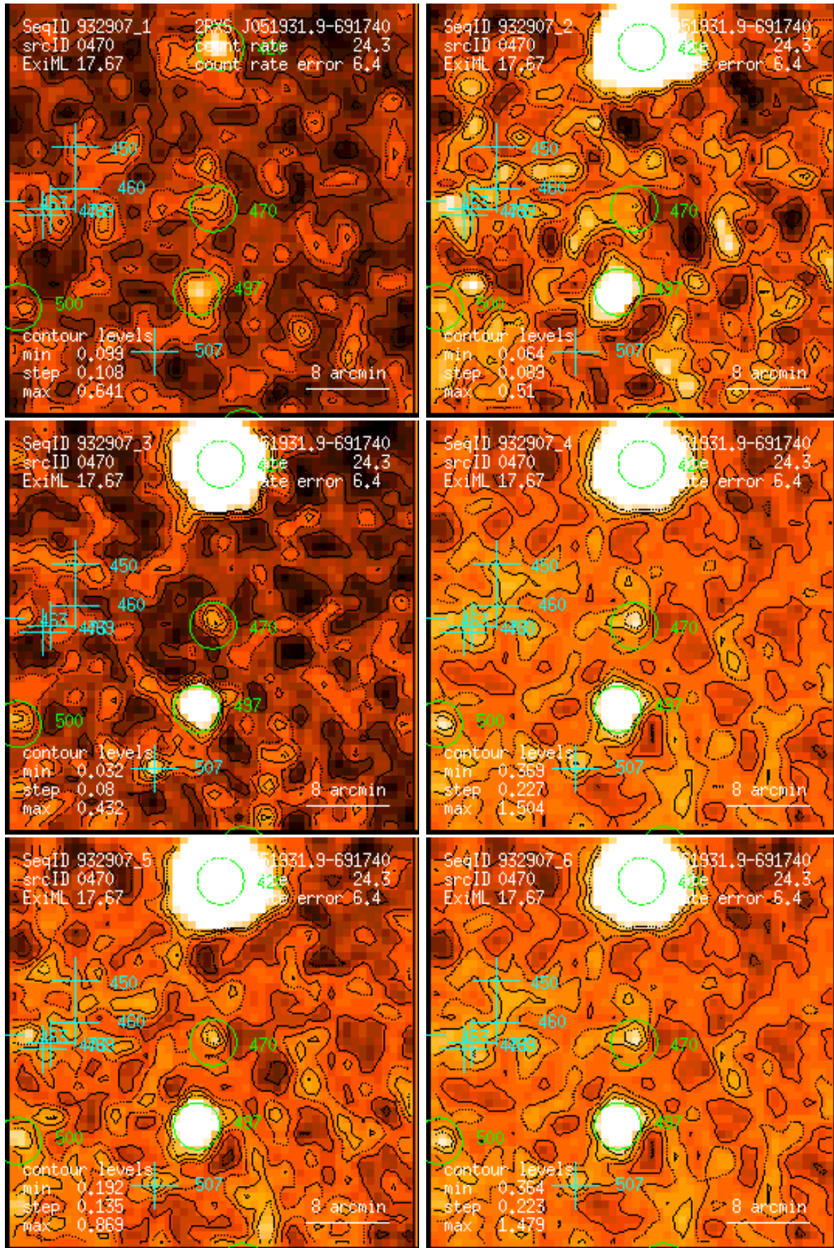
Figure 470: RASS 932907: detection 0470: band rate images, Gaussian filter: (1) PSPC channels 11 – 41, (2) 52 – 90, (3) 91 – 201, (4) 11 – 235, (5) 52 – 201, (6) 11 – 201. Broad band rates in counts/ks. Band rate contour levels in counts/ks/arcmin 2 .
