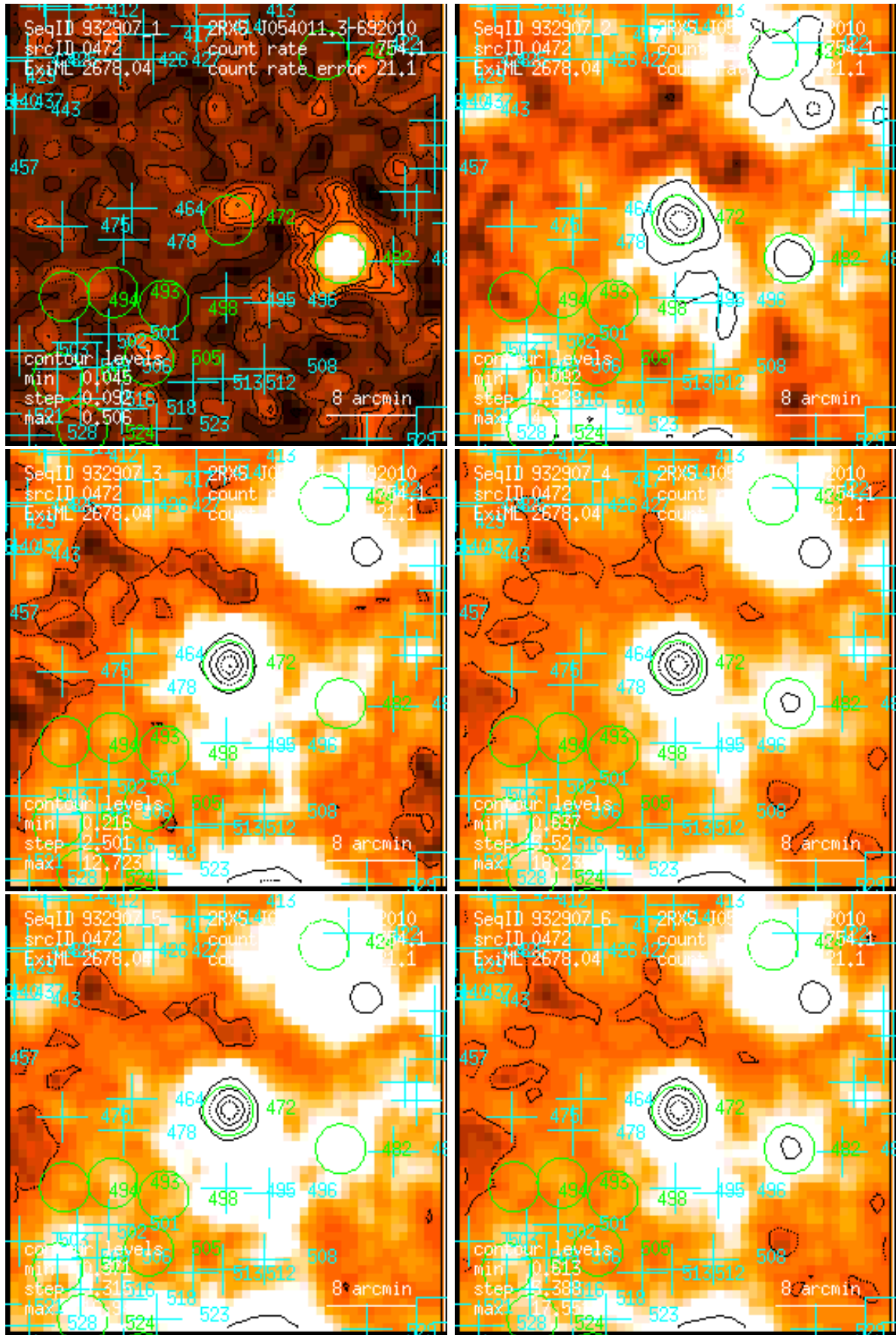
Figure 472: RASS 932907: detection 0472: band rate images, Gaussian filter: (1) PSPC channels 11 – 41, (2) 52 – 90, (3) 91 – 201, (4) 11 – 235, (5) 52 – 201, (6) 11 – 201. Broad band rates in counts/ks. Band rate contour levels in counts/ks/arcmin 2 .
