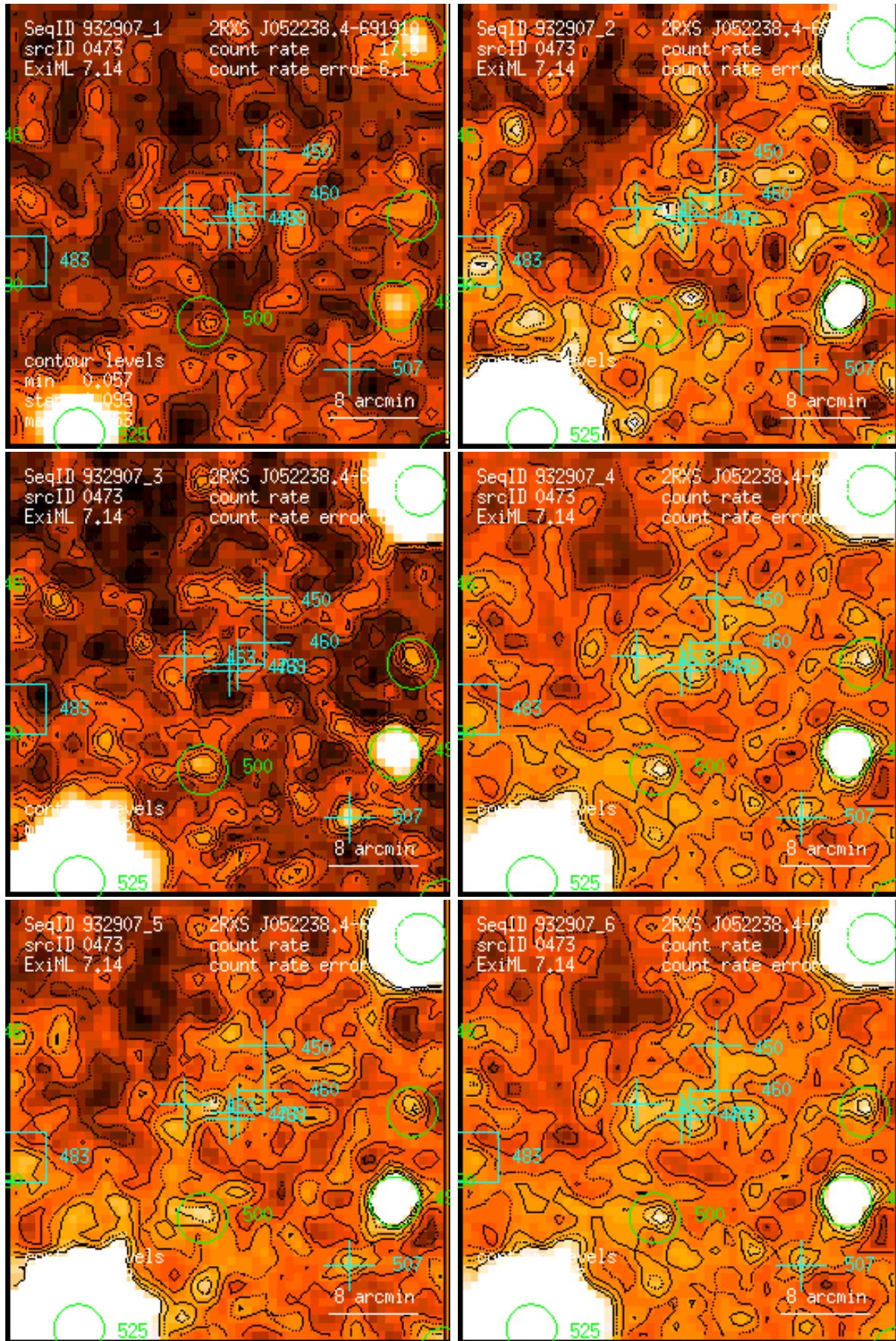
Figure 473: RASS 932907: detection 0473: band rate images, Gaussian filter: (1) PSPC channels 11 – 41, (2) 52 – 90, (3) 91 – 201, (4) 11 – 235, (5) 52 – 201, (6) 11 – 201. Broad band rates in counts/ks. Band rate contour levels in counts/ks/arcmin 2 .
