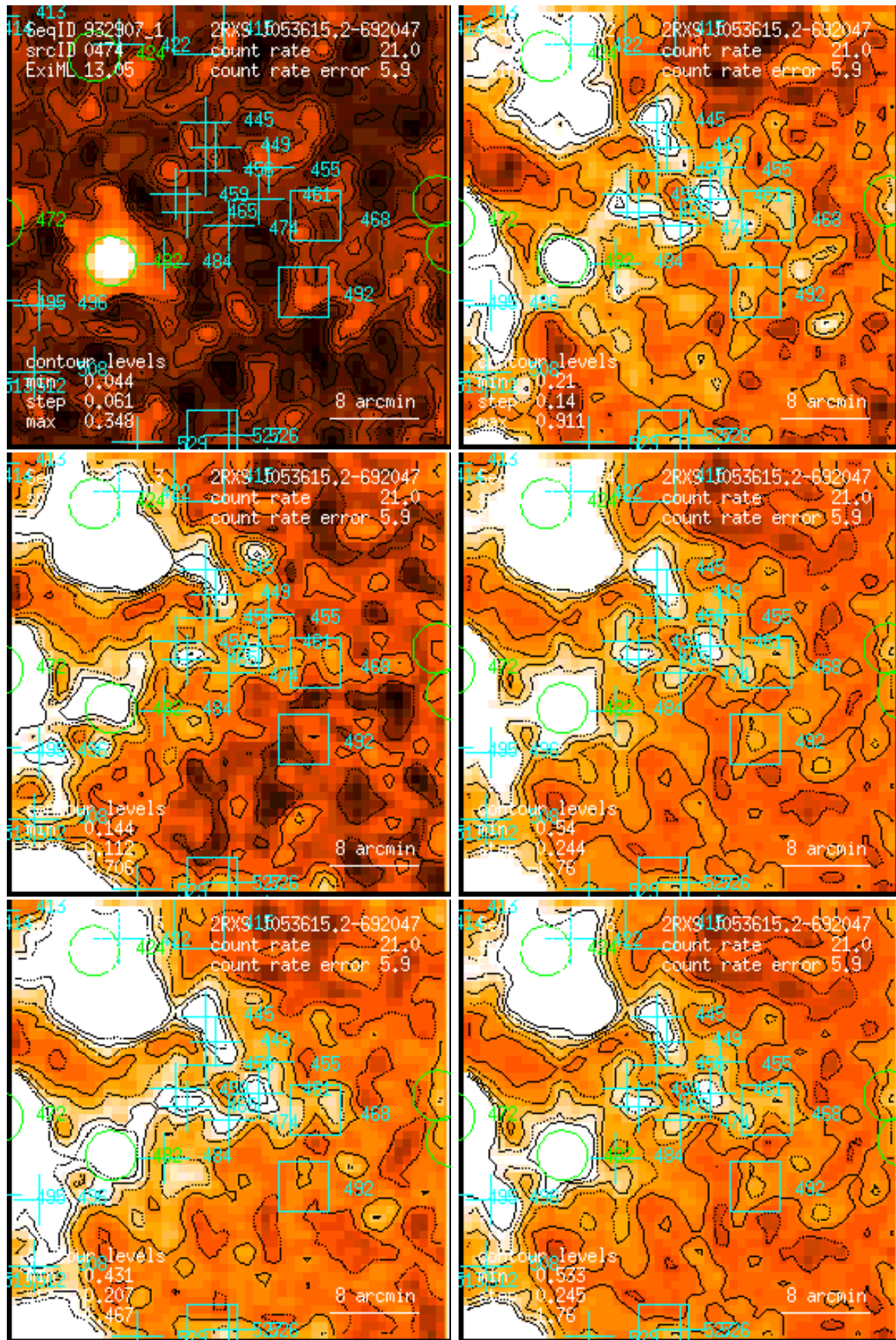
Figure 474: RASS 932907: detection 0474: band rate images, Gaussian filter: (1) PSPC channels 11 – 41, (2) 52 – 90, (3) 91 – 201, (4) 11 – 235, (5) 52 – 201, (6) 11 – 201. Broad band rates in counts/ks. Band rate contour levels in counts/ks/arcmin 2 .
