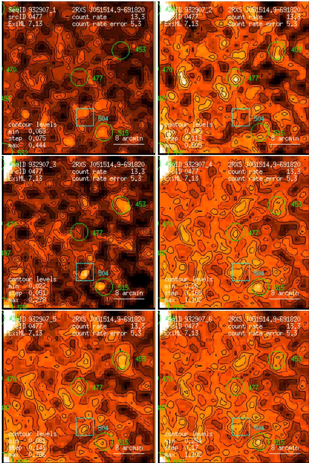
Figure 477: RASS 932907: detection 0477: band rate images, Gaussian filter: (1) PSPC channels 11 – 41, (2) 52 – 90, (3) 91 – 201, (4) 11 – 235, (5) 52 – 201, (6) 11 – 201. Broad band rates in counts/ks. Band rate contour levels in counts/ks/arcmin 2 .
