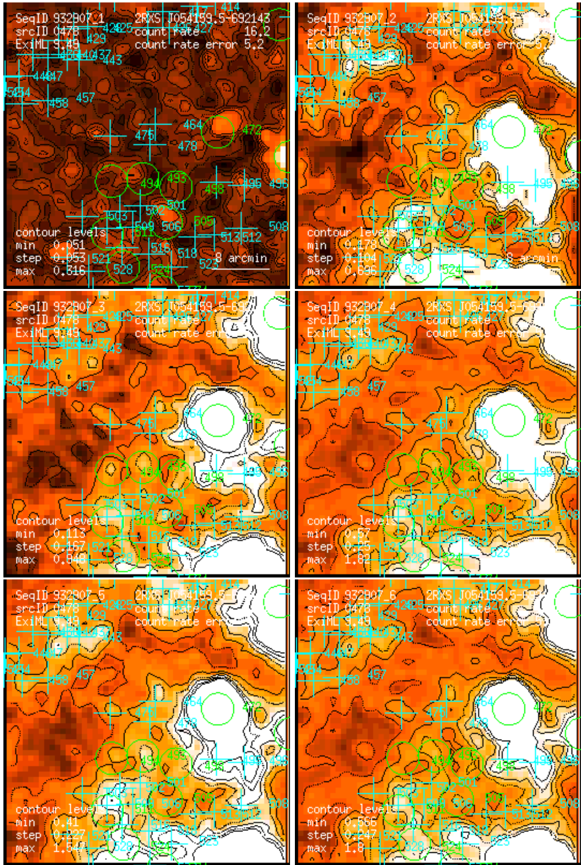
Figure 478: RASS 932907: detection 0478: band rate images, Gaussian filter: (1) PSPC channels 11 – 41, (2) 52 – 90, (3) 91 – 201, (4) 11 – 235, (5) 52 – 201, (6) 11 – 201. Broad band rates in counts/ks. Band rate contour levels in counts/ks/arcmin 2 .
