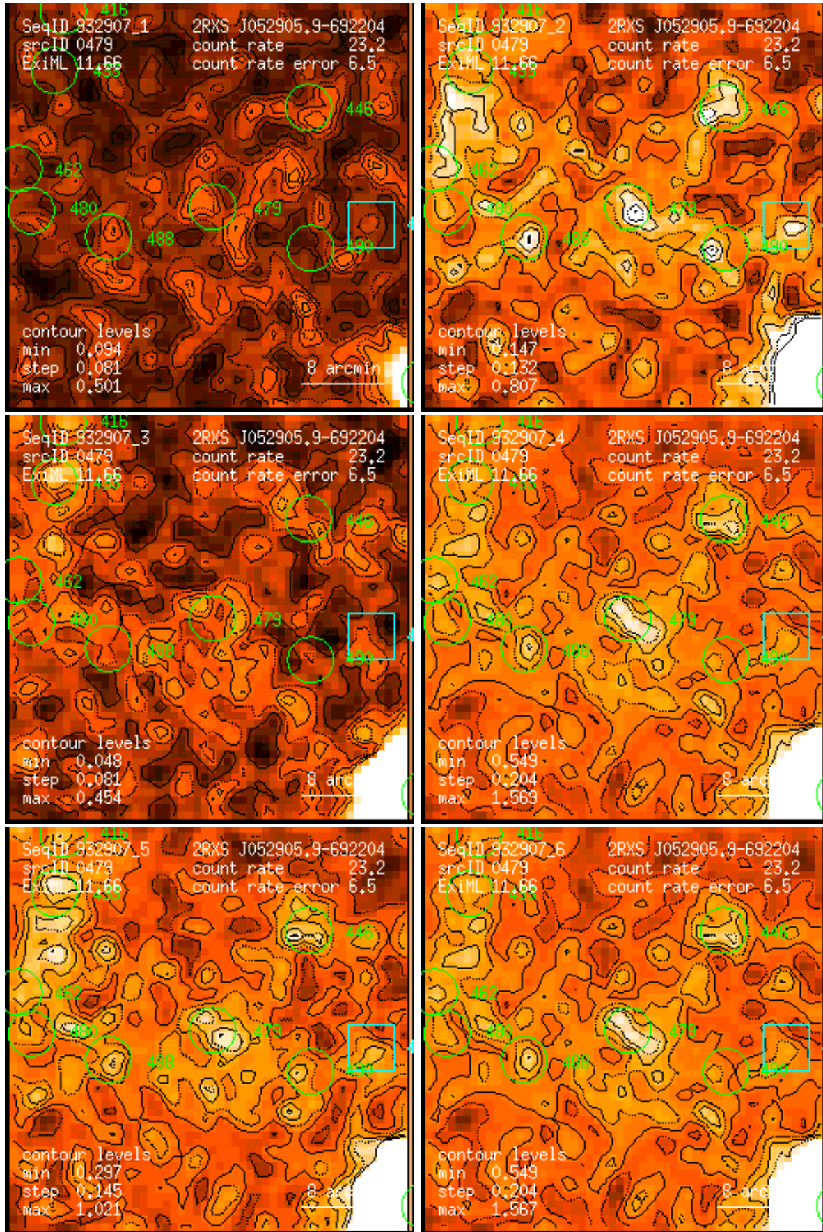
Figure 479: RASS 932907: detection 0479: band rate images, Gaussian filter: (1) PSPC channels 11 – 41, (2) 52 – 90, (3) 91 – 201, (4) 11 – 235, (5) 52 – 201, (6) 11 – 201. Broad band rates in counts/ks. Band rate contour levels in counts/ks/arcmin 2 .
