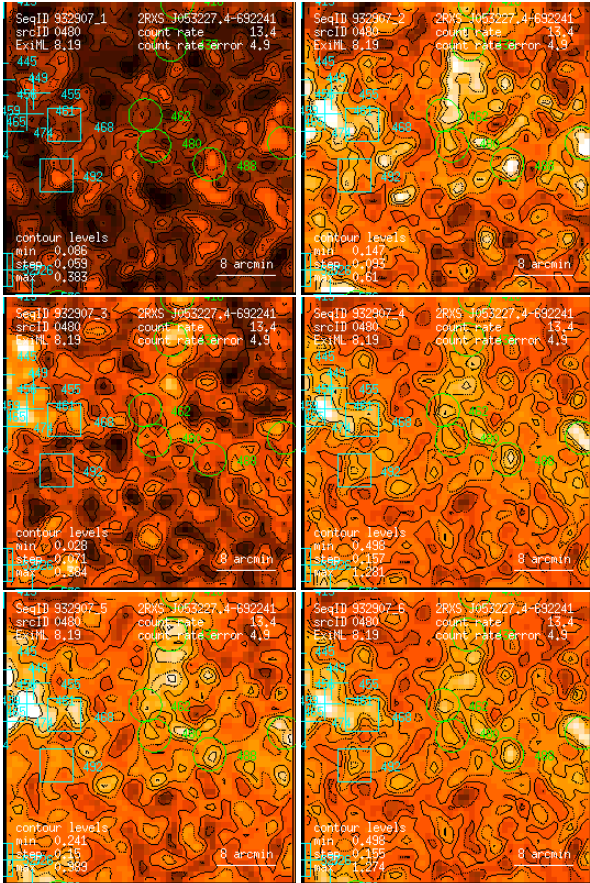
Figure 480: RASS 932907: detection 0480: band rate images, Gaussian filter: (1) PSPC channels 11 – 41, (2) 52 – 90, (3) 91 – 201, (4) 11 – 235, (5) 52 – 201, (6) 11 – 201. Broad band rates in counts/ks. Band rate contour levels in counts/ks/arcmin 2 .
