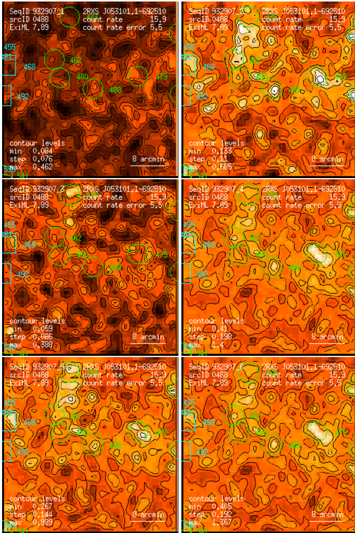
Figure 488: RASS 932907: detection 0488: band rate images, Gaussian filter: (1) PSPC channels 11 – 41, (2) 52 – 90, (3) 91 – 201, (4) 11 – 235, (5) 52 – 201, (6) 11 – 201. Broad band rates in counts/ks. Band rate contour levels in counts/ks/arcmin 2 .
