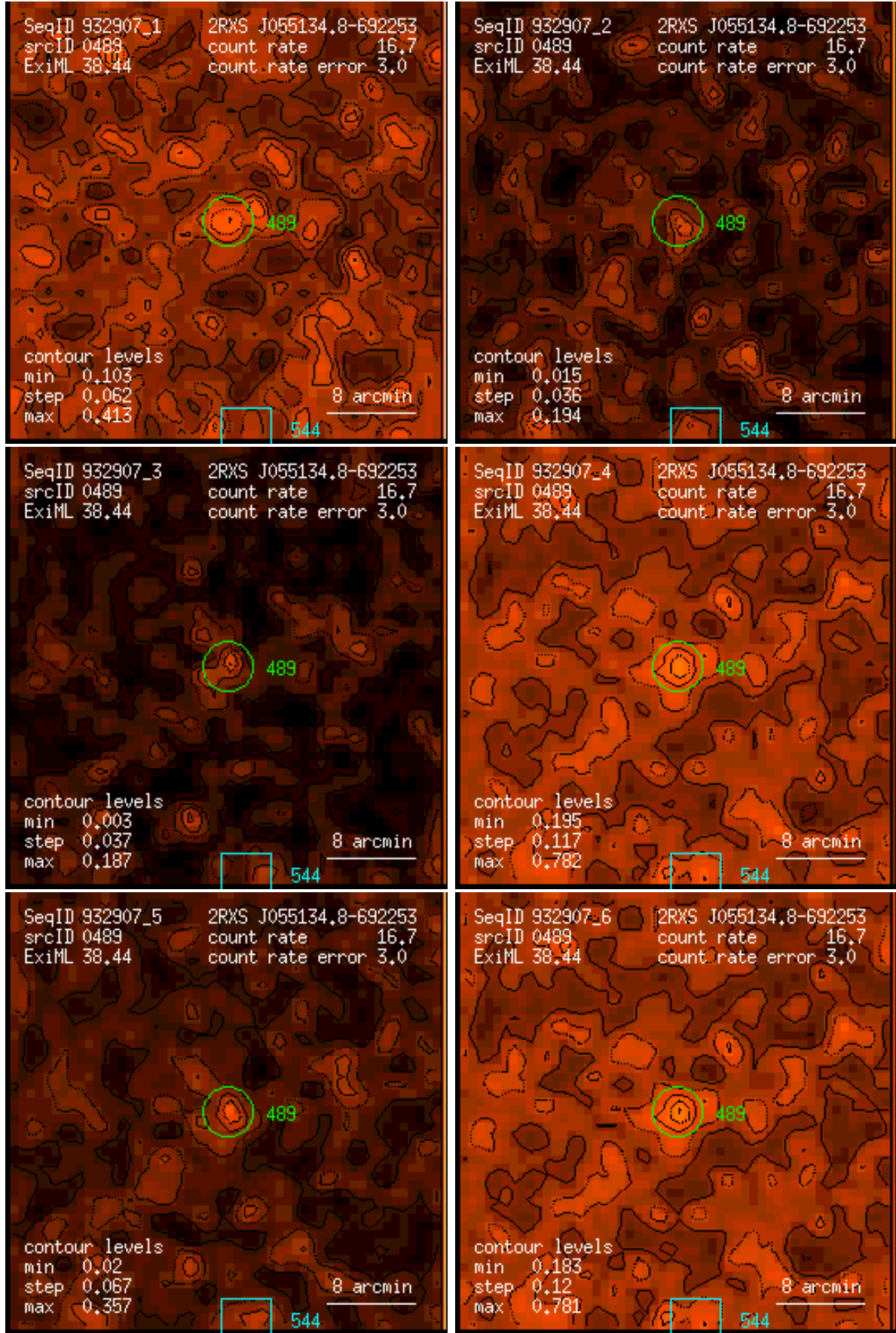
Figure 489: RASS 932907: detection 0489: band rate images, Gaussian filter: (1) PSPC channels 11 – 41, (2) 52 – 90, (3) 91 – 201, (4) 11 – 235, (5) 52 – 201, (6) 11 – 201. Broad band rates in counts/ks. Band rate contour levels in counts/ks/arcmin 2 .
