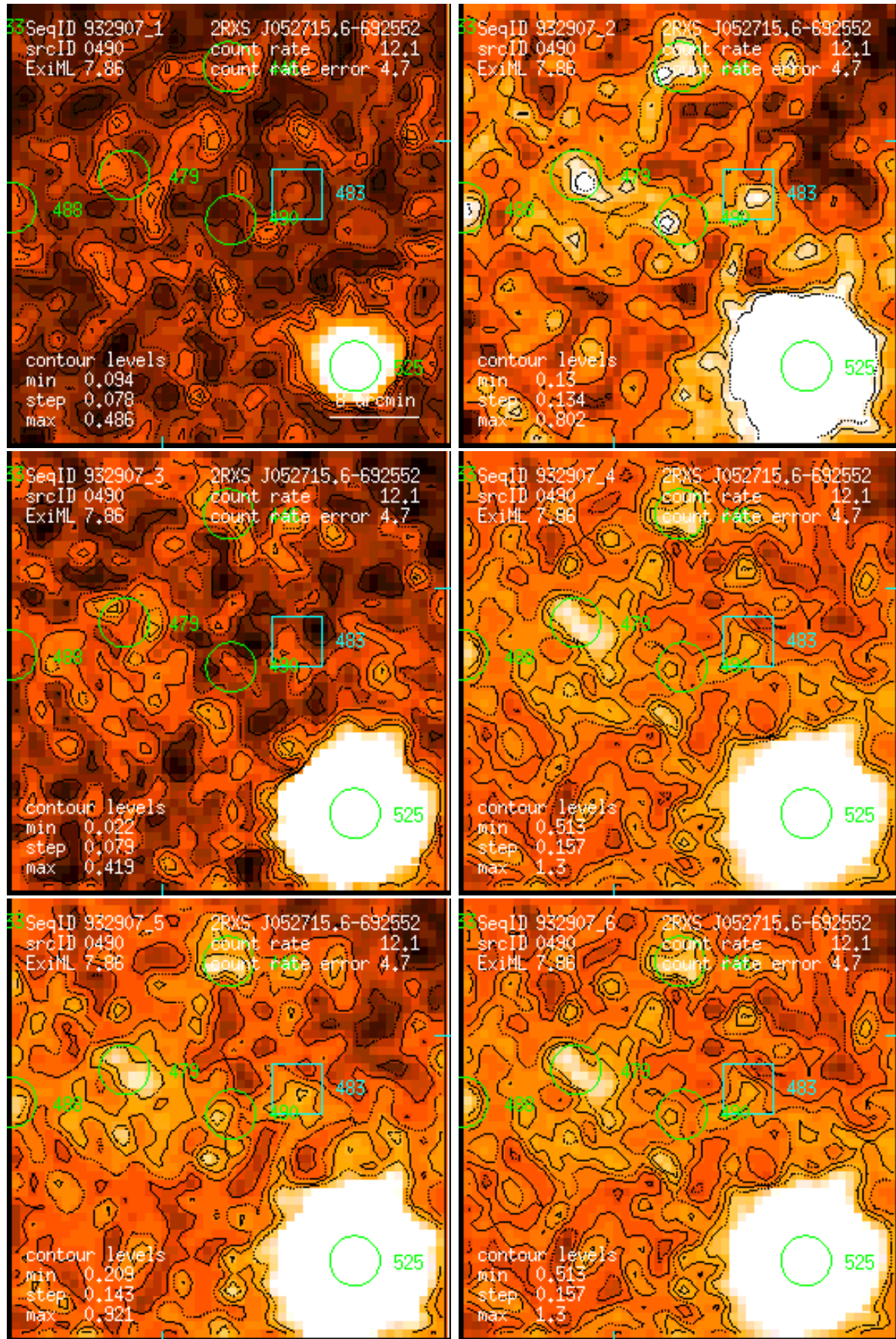
Figure 490: RASS 932907: detection 0490: band rate images, Gaussian filter: (1) PSPC channels 11 – 41, (2) 52 – 90, (3) 91 – 201, (4) 11 – 235, (5) 52 – 201, (6) 11 – 201. Broad band rates in counts/ks. Band rate contour levels in counts/ks/arcmin 2 .
