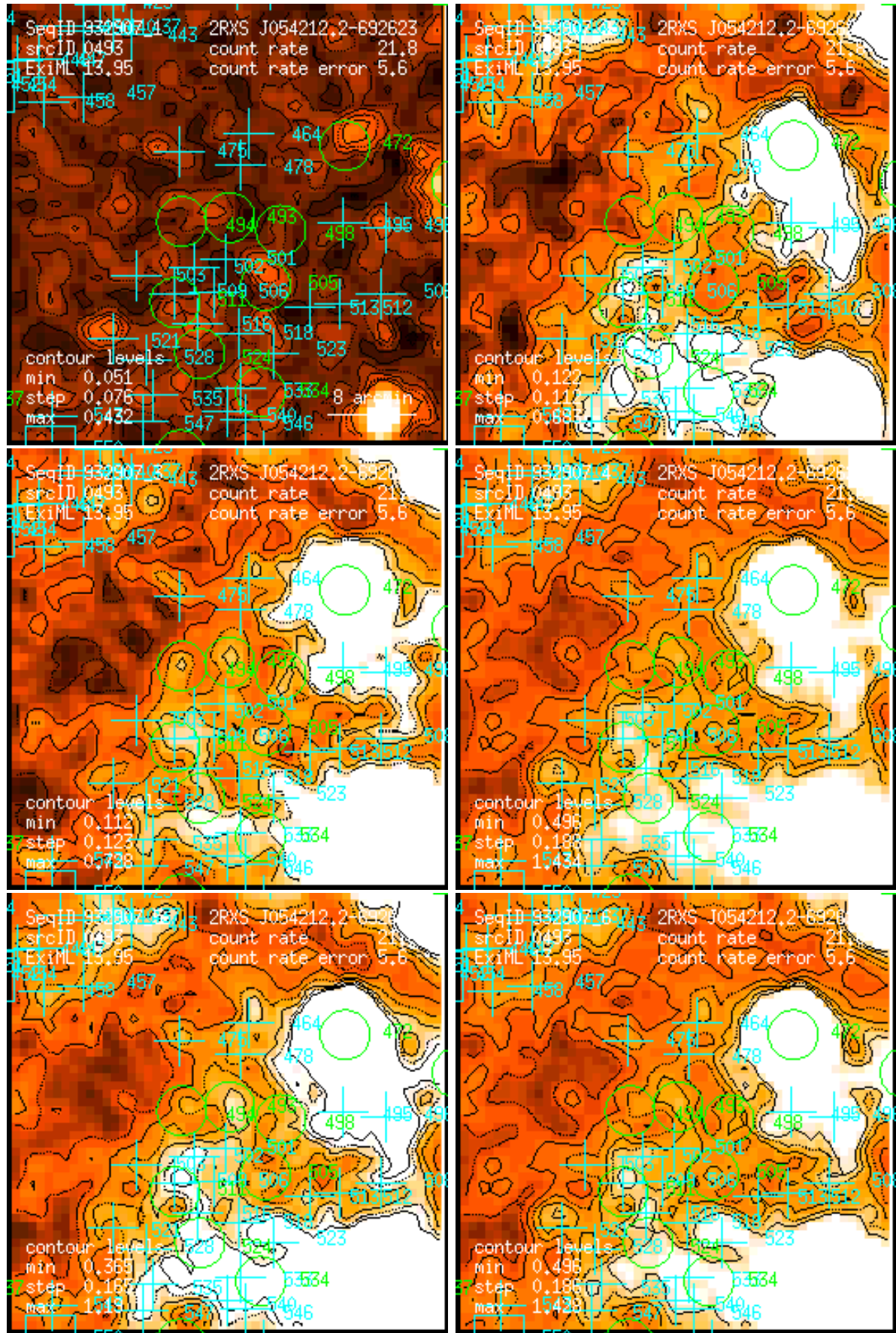
Figure 493: RASS 932907: detection 0493: band rate images, Gaussian filter: (1) PSPC channels 11 – 41, (2) 52 – 90, (3) 91 – 201, (4) 11 – 235, (5) 52 – 201, (6) 11 – 201. Broad band rates in counts/ks. Band rate contour levels in counts/ks/arcmin 2 .
