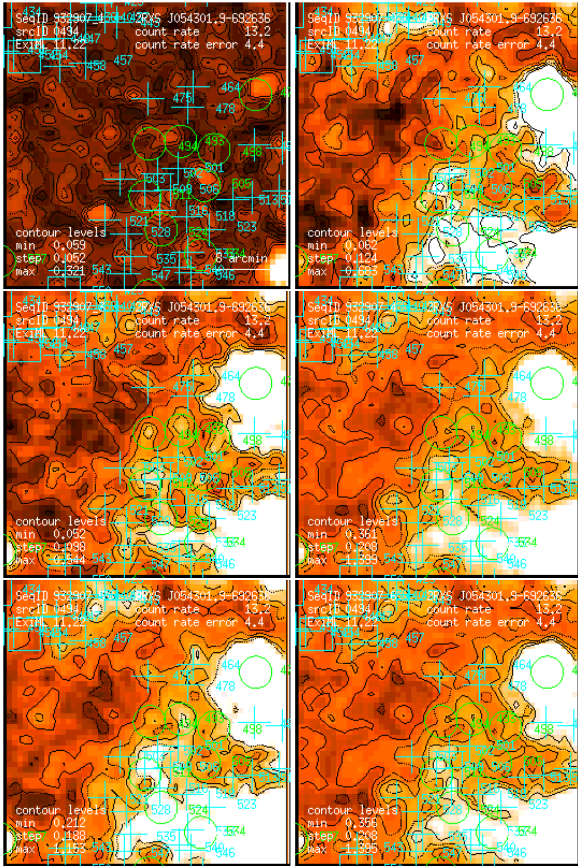
Figure 494: RASS 932907: detection 0494: band rate images, Gaussian filter: (1) PSPC channels 11 – 41, (2) 52 – 90, (3) 91 – 201, (4) 11 – 235, (5) 52 – 201, (6) 11 – 201. Broad band rates in counts/ks. Band rate contour levels in counts/ks/arcmin 2 .
