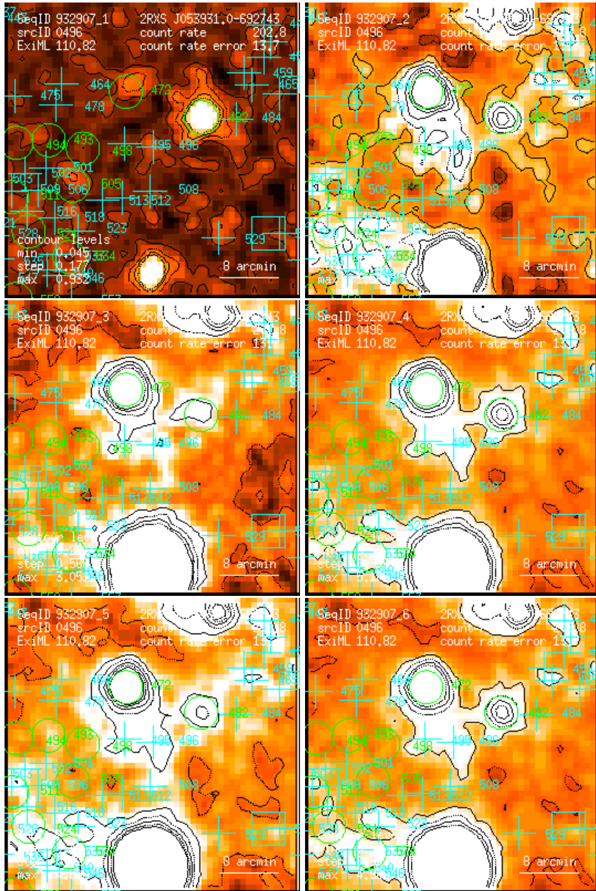
Figure 496: RASS 932907: detection 0496: band rate images, Gaussian filter: (1) PSPC channels 11 – 41, (2) 52 – 90, (3) 91 – 201, (4) 11 – 235, (5) 52 – 201, (6) 11 – 201. Broad band rates in counts/ks. Band rate contour levels in counts/ks/arcmin 2 .
