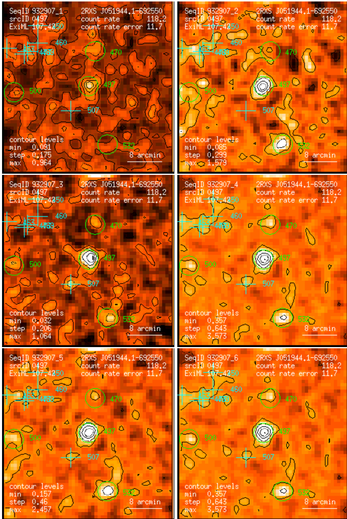
Figure 497: RASS 932907: detection 0497: band rate images, Gaussian filter: (1) PSPC channels 11 – 41, (2) 52 – 90, (3) 91 – 201, (4) 11 – 235, (5) 52 – 201, (6) 11 – 201. Broad band rates in counts/ks. Band rate contour levels in counts/ks/arcmin 2 .
