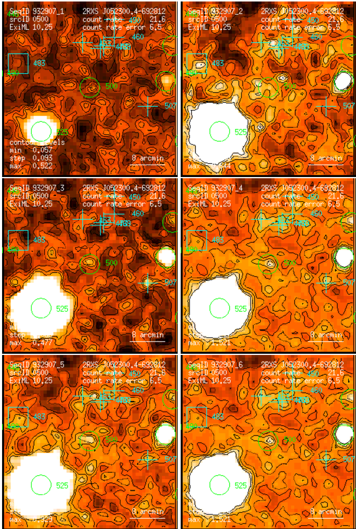
Figure 500: RASS 932907: detection 0500: band rate images, Gaussian filter: (1) PSPC channels 11 – 41, (2) 52 – 90, (3) 91 – 201, (4) 11 – 235, (5) 52 – 201, (6) 11 – 201. Broad band rates in counts/ks. Band rate contour levels in counts/ks/arcmin 2 .
