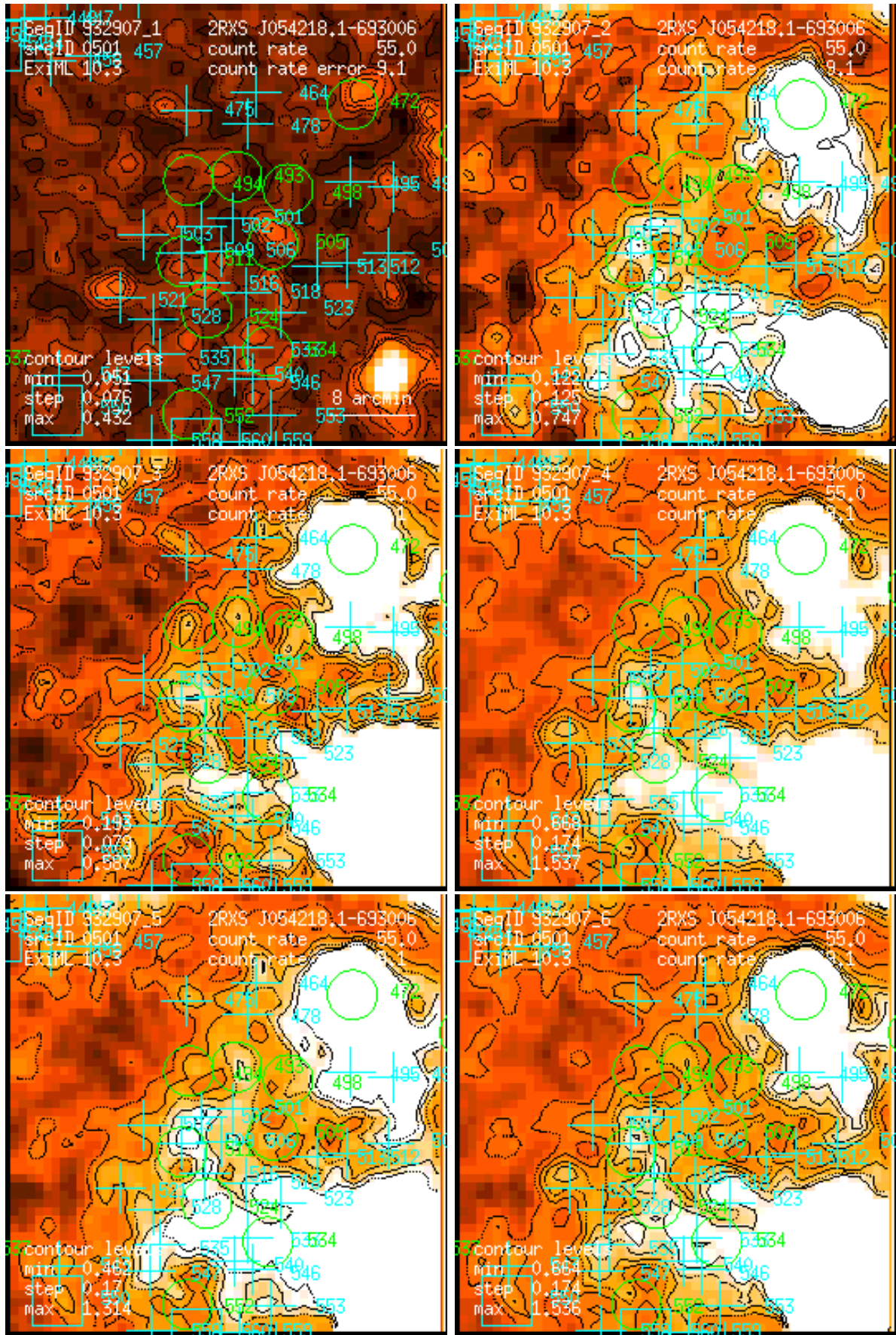
Figure 501: RASS 932907: detection 0501: band rate images, Gaussian filter: (1) PSPC channels 11 – 41, (2) 52 – 90, (3) 91 – 201, (4) 11 – 235, (5) 52 – 201, (6) 11 – 201. Broad band rates in counts/ks. Band rate contour levels in counts/ks/arcmin 2 .
