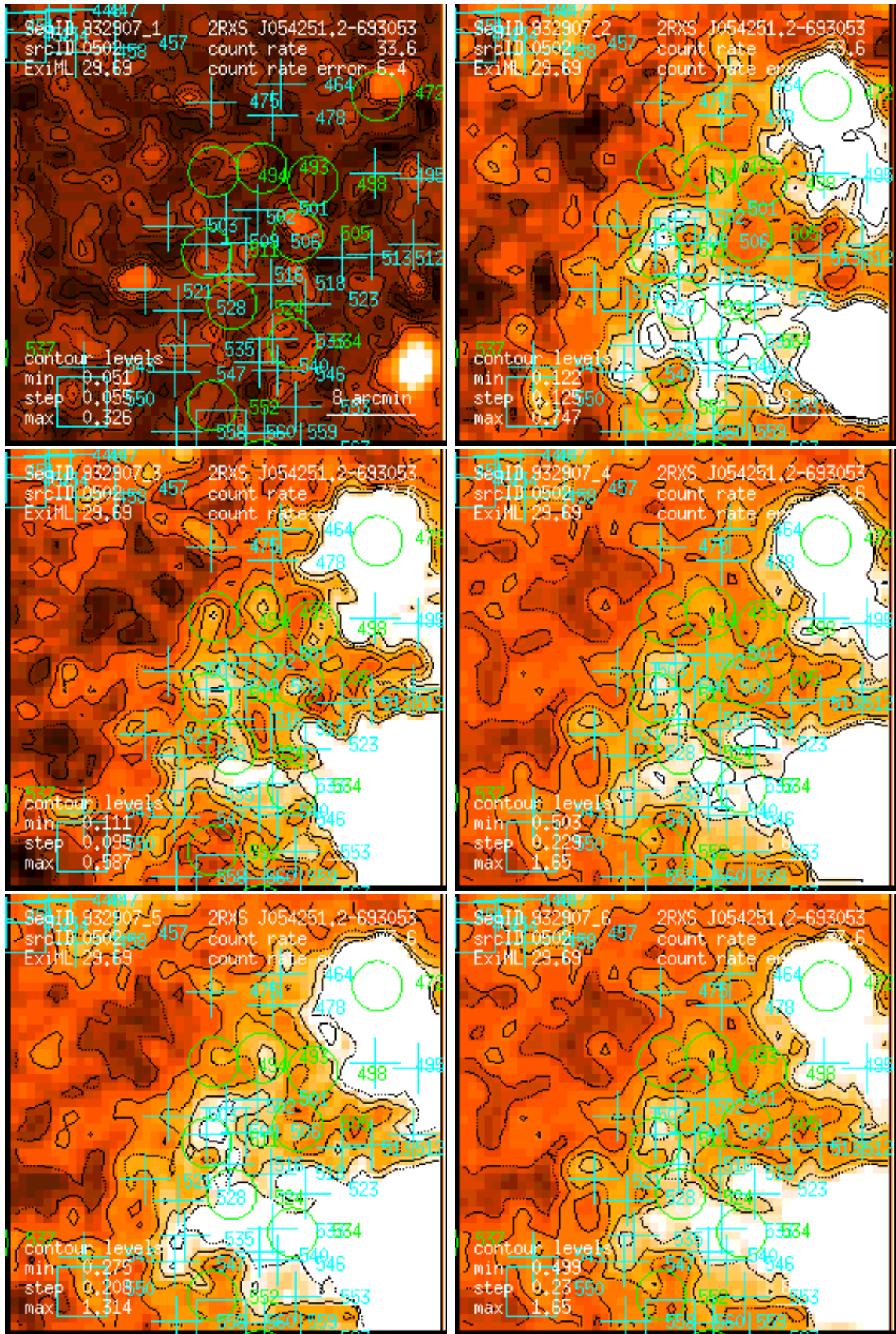
Figure 502: RASS 932907: detection 0502: band rate images, Gaussian filter: (1) PSPC channels 11 – 41, (2) 52 – 90, (3) 91 – 201, (4) 11 – 235, (5) 52 – 201, (6) 11 – 201. Broad band rates in counts/ks. Band rate contour levels in counts/ks/arcmin 2 .
