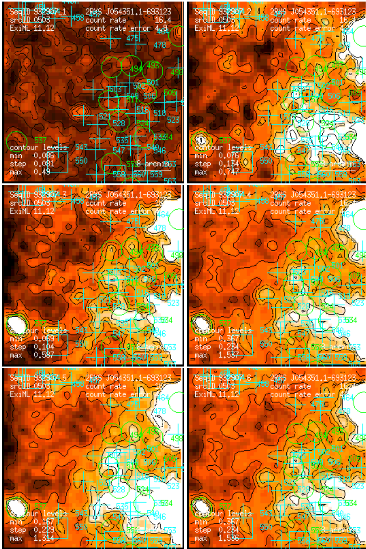
Figure 503: RASS 932907: detection 0503: band rate images, Gaussian filter: (1) PSPC channels 11 – 41, (2) 52 – 90, (3) 91 – 201, (4) 11 – 235, (5) 52 – 201, (6) 11 – 201. Broad band rates in counts/ks. Band rate contour levels in counts/ks/arcmin 2 .
