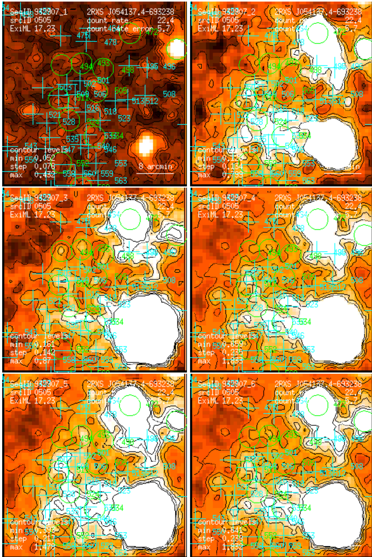
Figure 505: RASS 932907: detection 0505: band rate images, Gaussian filter: (1) PSPC channels 11 – 41, (2) 52 – 90, (3) 91 – 201, (4) 11 – 235, (5) 52 – 201, (6) 11 – 201. Broad band rates in counts/ks. Band rate contour levels in counts/ks/arcmin 2 .
