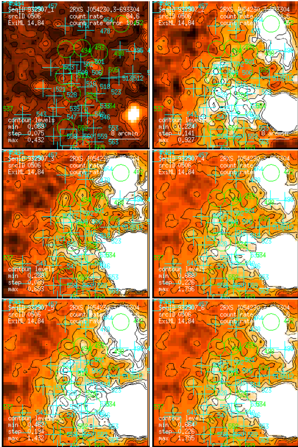
Figure 506: RASS 932907: detection 0506: band rate images, Gaussian filter: (1) PSPC channels 11 – 41, (2) 52 – 90, (3) 91 – 201, (4) 11 – 235, (5) 52 – 201, (6) 11 – 201. Broad band rates in counts/ks. Band rate contour levels in counts/ks/arcmin 2 .
