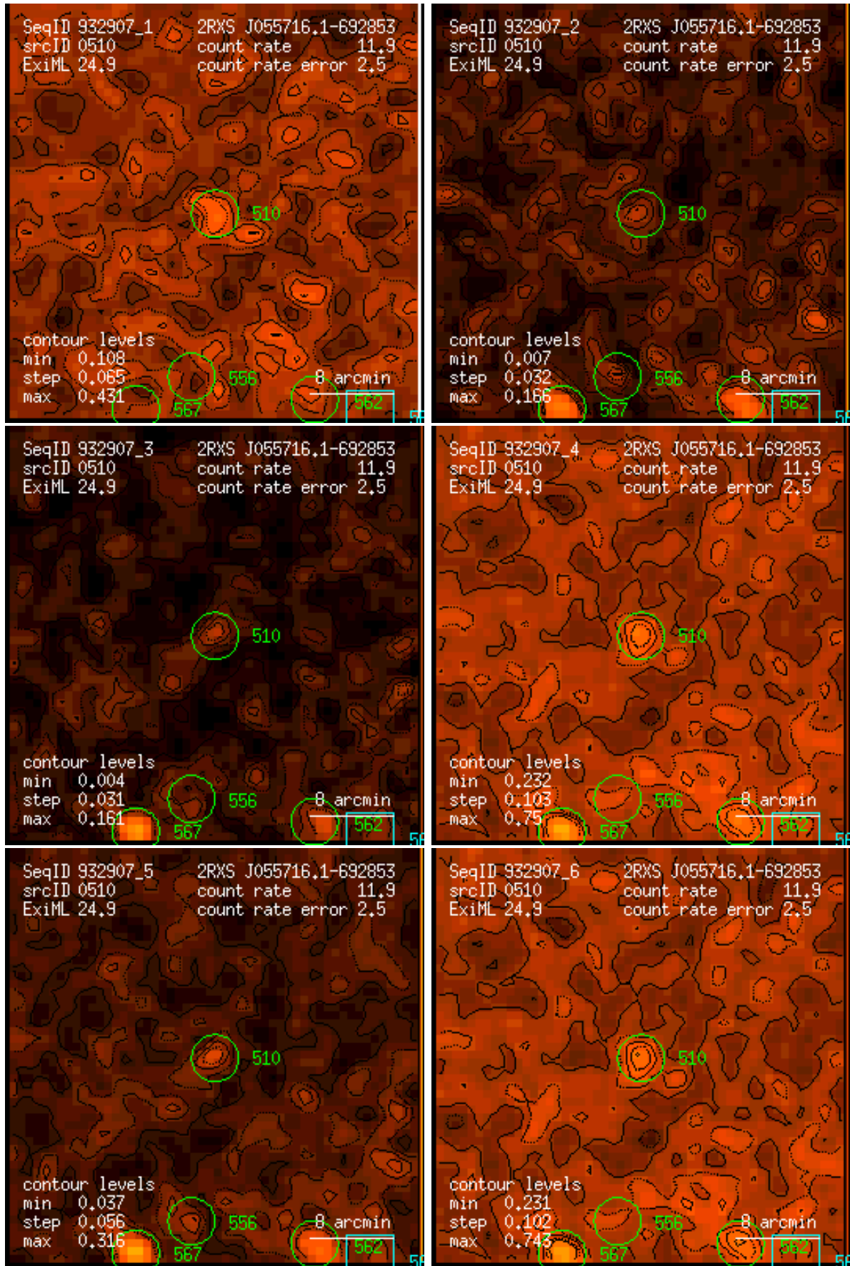
Figure 510: RASS 932907: detection 0510: band rate images, Gaussian filter: (1) PSPC channels 11 – 41, (2) 52 – 90, (3) 91 – 201, (4) 11 – 235, (5) 52 – 201, (6) 11 – 201. Broad band rates in counts/ks. Band rate contour levels in counts/ks/arcmin 2 .
