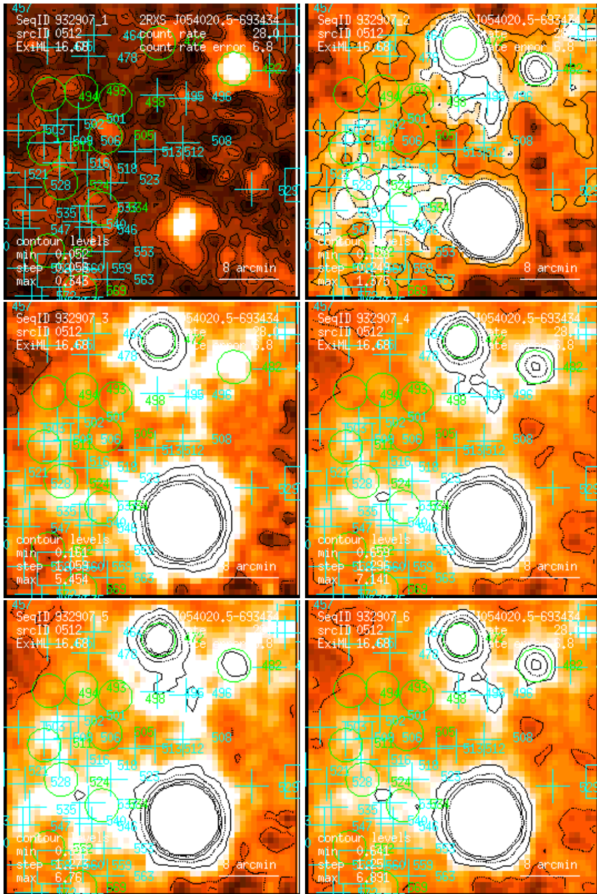
Figure 512: RASS 932907: detection 0512: band rate images, Gaussian filter: (1) PSPC channels 11 – 41, (2) 52 – 90, (3) 91 – 201, (4) 11 – 235, (5) 52 – 201, (6) 11 – 201. Broad band rates in counts/ks. Band rate contour levels in counts/ks/arcmin 2 .
