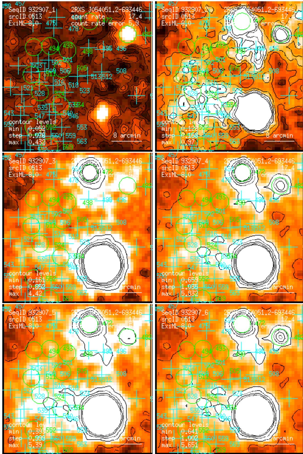
Figure 513: RASS 932907: detection 0513: band rate images, Gaussian filter: (1) PSPC channels 11 – 41, (2) 52 – 90, (3) 91 – 201, (4) 11 – 235, (5) 52 – 201, (6) 11 – 201. Broad band rates in counts/ks. Band rate contour levels in counts/ks/arcmin 2 .
