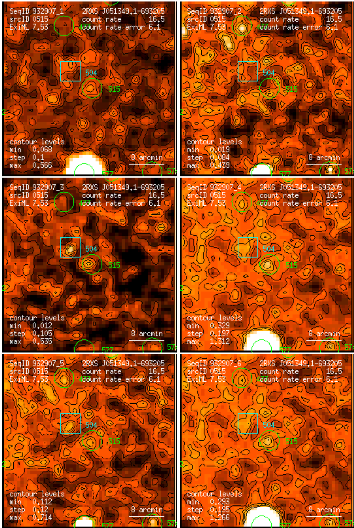
Figure 515: RASS 932907: detection 0515: band rate images, Gaussian filter: (1) PSPC channels 11 – 41, (2) 52 – 90, (3) 91 – 201, (4) 11 – 235, (5) 52 – 201, (6) 11 – 201. Broad band rates in counts/ks. Band rate contour levels in counts/ks/arcmin 2 .
