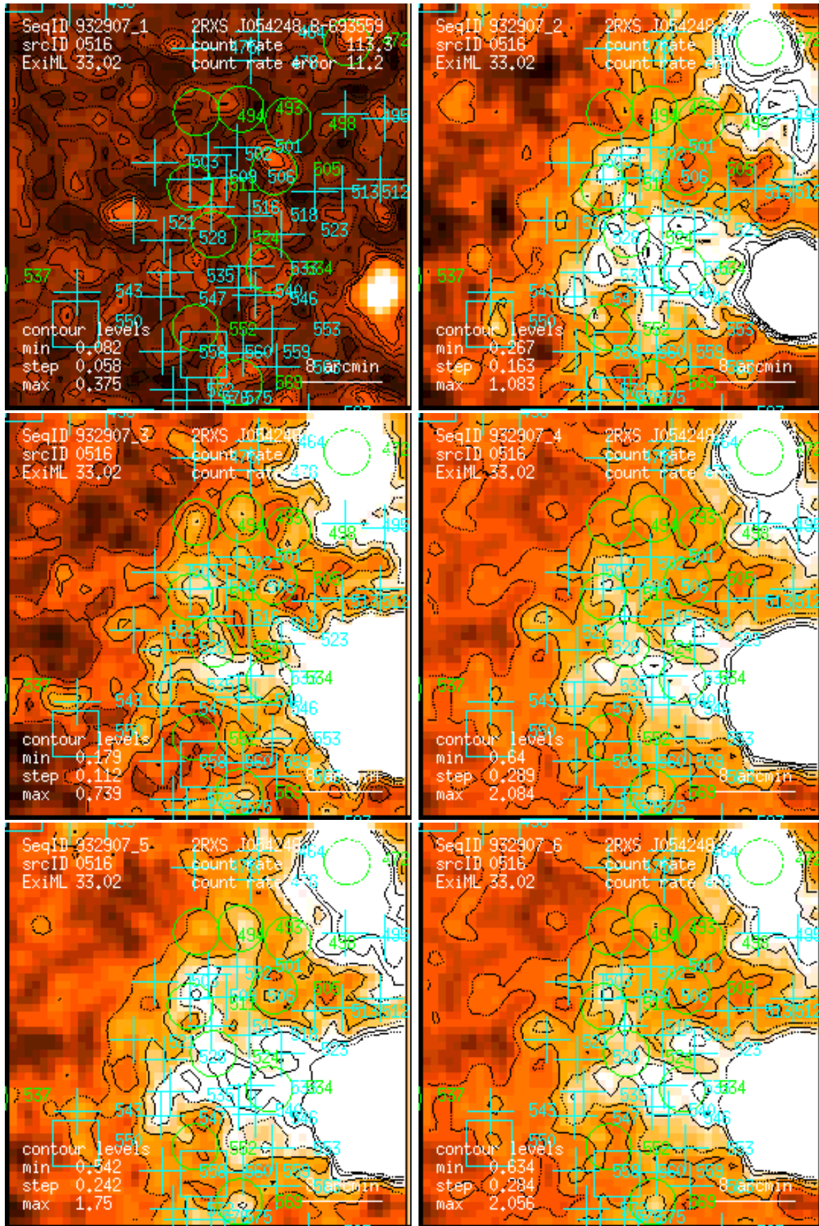
Figure 516: RASS 932907: detection 0516: band rate images, Gaussian filter: (1) PSPC channels 11 – 41, (2) 52 – 90, (3) 91 – 201, (4) 11 – 235, (5) 52 – 201, (6) 11 – 201. Broad band rates in counts/ks. Band rate contour levels in counts/ks/arcmin 2 .
