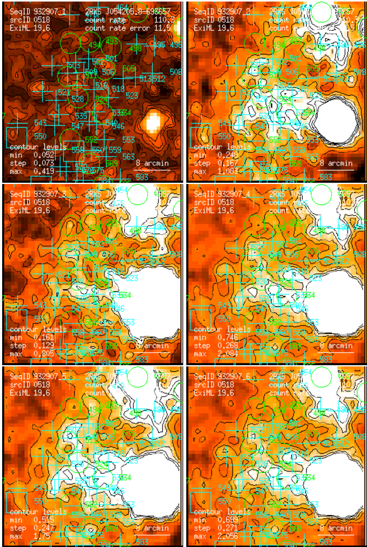
Figure 518: RASS 932907: detection 0518: band rate images, Gaussian filter: (1) PSPC channels 11 – 41, (2) 52 – 90, (3) 91 – 201, (4) 11 – 235, (5) 52 – 201, (6) 11 – 201. Broad band rates in counts/ks. Band rate contour levels in counts/ks/arcmin 2 .
