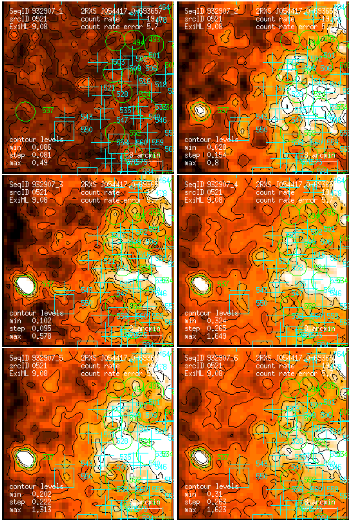
Figure 521: RASS 932907: detection 0521: band rate images, Gaussian filter: (1) PSPC channels 11 – 41, (2) 52 – 90, (3) 91 – 201, (4) 11 – 235, (5) 52 – 201, (6) 11 – 201. Broad band rates in counts/ks. Band rate contour levels in counts/ks/arcmin 2 .
