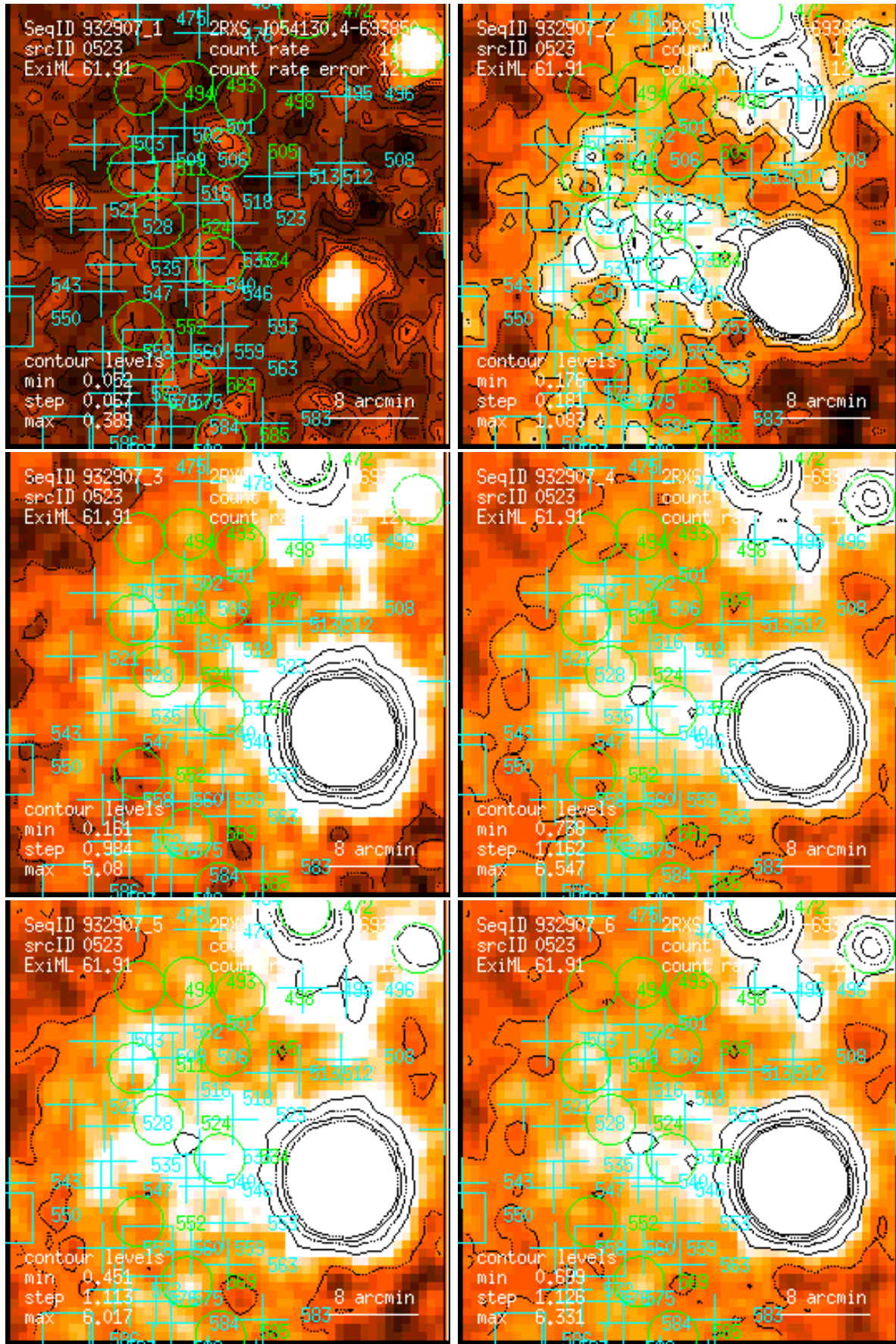
Figure 523: RASS 932907: detection 0523: band rate images, Gaussian filter: (1) PSPC channels 11 – 41, (2) 52 – 90, (3) 91 – 201, (4) 11 – 235, (5) 52 – 201, (6) 11 – 201. Broad band rates in counts/ks. Band rate contour levels in counts/ks/arcmin 2 .
