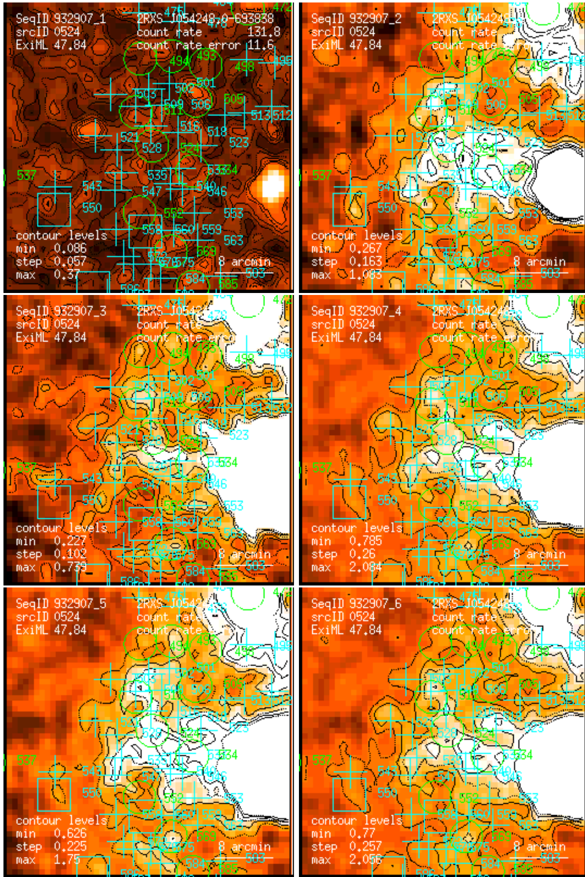
Figure 524: RASS 932907: detection 0524: band rate images, Gaussian filter: (1) PSPC channels 11 – 41, (2) 52 – 90, (3) 91 – 201, (4) 11 – 235, (5) 52 – 201, (6) 11 – 201. Broad band rates in counts/ks. Band rate contour levels in counts/ks/arcmin 2 .
