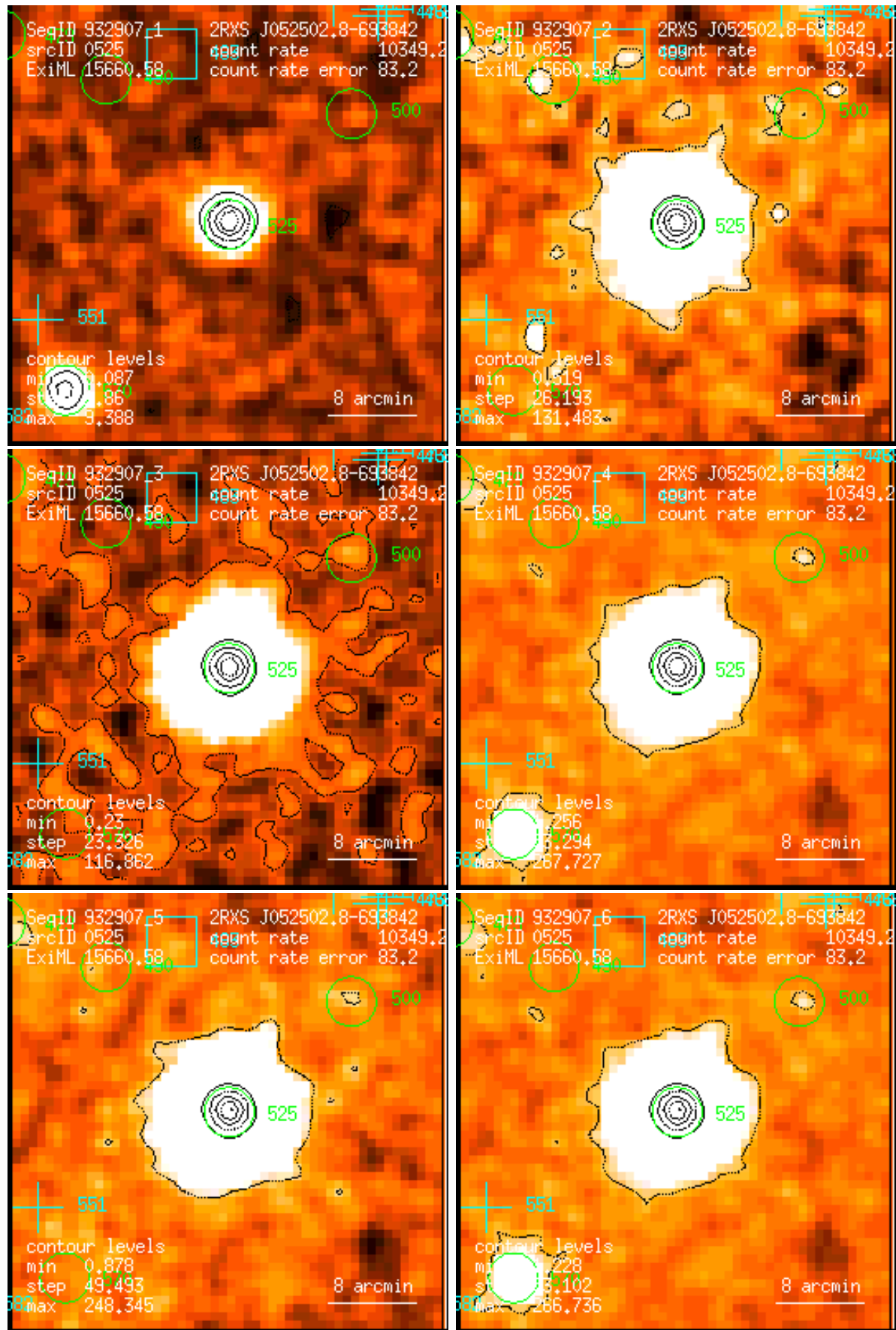
Figure 525: RASS 932907: detection 0525: band rate images, Gaussian filter: (1) PSPC channels 11 – 41, (2) 52 – 90, (3) 91 – 201, (4) 11 – 235, (5) 52 – 201, (6) 11 – 201. Broad band rates in counts/ks. Band rate contour levels in counts/ks/arcmin 2 .
