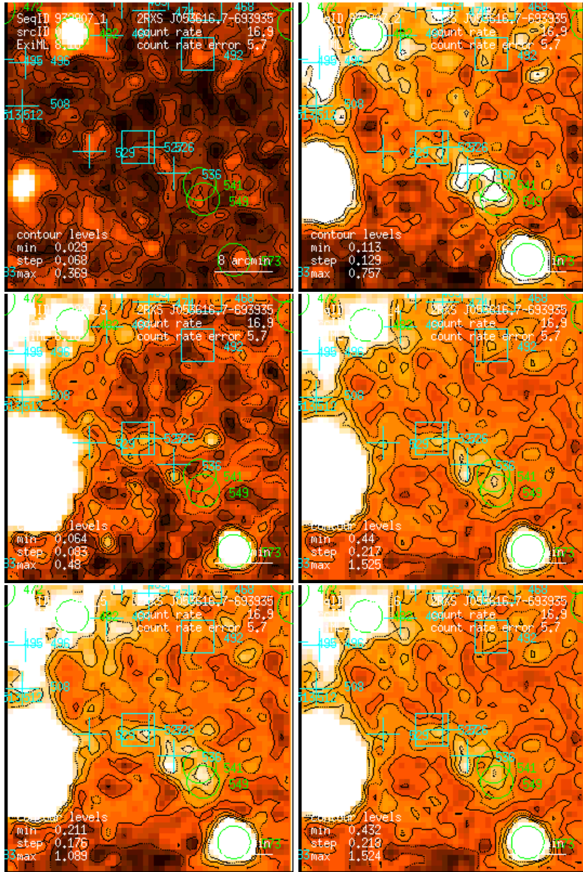
Figure 526: RASS 932907: detection 0526: band rate images, Gaussian filter: (1) PSPC channels 11 – 41, (2) 52 – 90, (3) 91 – 201, (4) 11 – 235, (5) 52 – 201, (6) 11 – 201. Broad band rates in counts/ks. Band rate contour levels in counts/ks/arcmin 2 .
