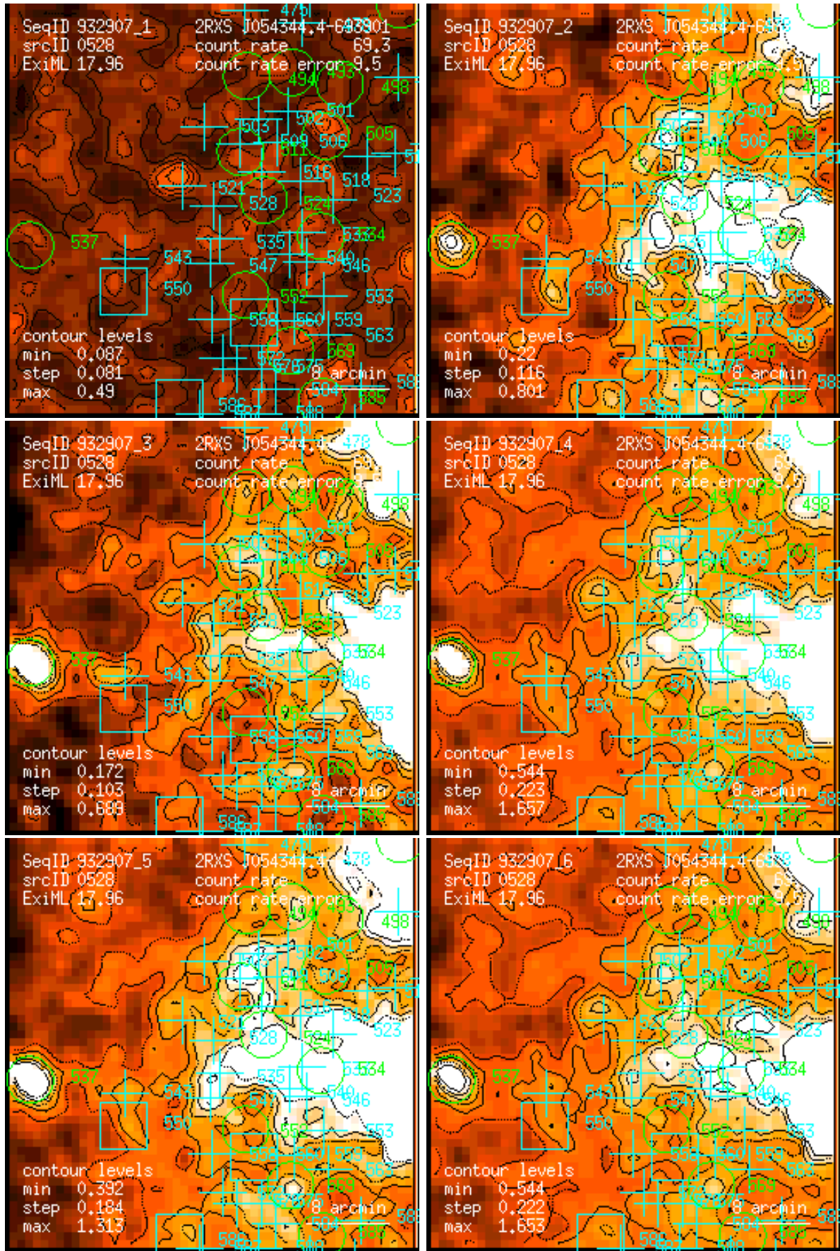
Figure 528: RASS 932907: detection 0528: band rate images, Gaussian filter: (1) PSPC channels 11 – 41, (2) 52 – 90, (3) 91 – 201, (4) 11 – 235, (5) 52 – 201, (6) 11 – 201. Broad band rates in counts/ks. Band rate contour levels in counts/ks/arcmin 2 .
