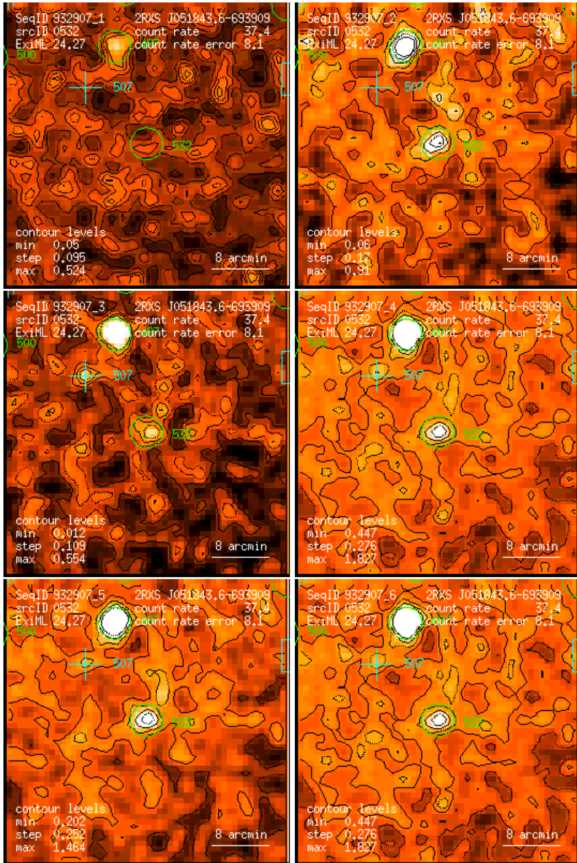
Figure 532: RASS 932907: detection 0532: band rate images, Gaussian filter: (1) PSPC channels 11 – 41, (2) 52 – 90, (3) 91 – 201, (4) 11 – 235, (5) 52 – 201, (6) 11 – 201. Broad band rates in counts/ks. Band rate contour levels in counts/ks/arcmin 2 .
