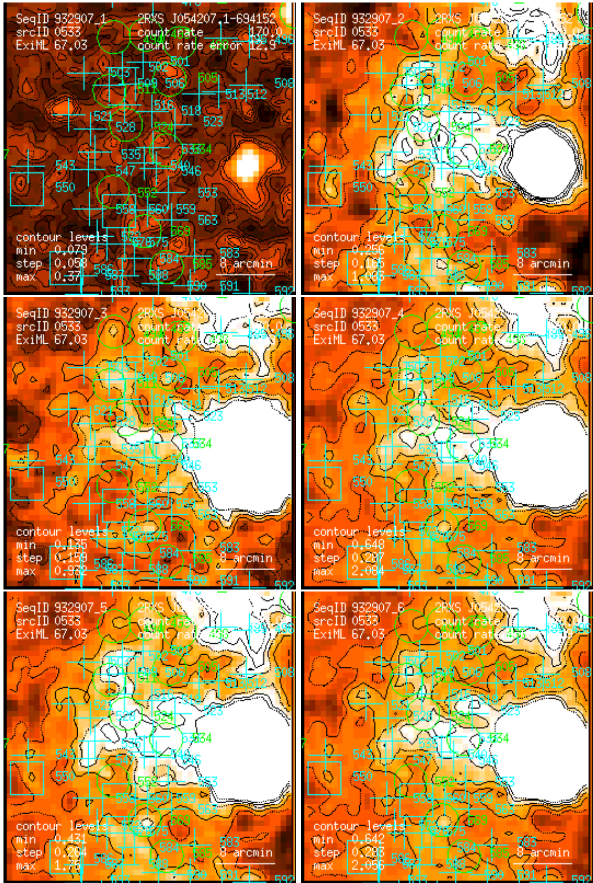
Figure 533: RASS 932907: detection 0533: band rate images, Gaussian filter: (1) PSPC channels 11 – 41, (2) 52 – 90, (3) 91 – 201, (4) 11 – 235, (5) 52 – 201, (6) 11 – 201. Broad band rates in counts/ks. Band rate contour levels in counts/ks/arcmin 2 .
