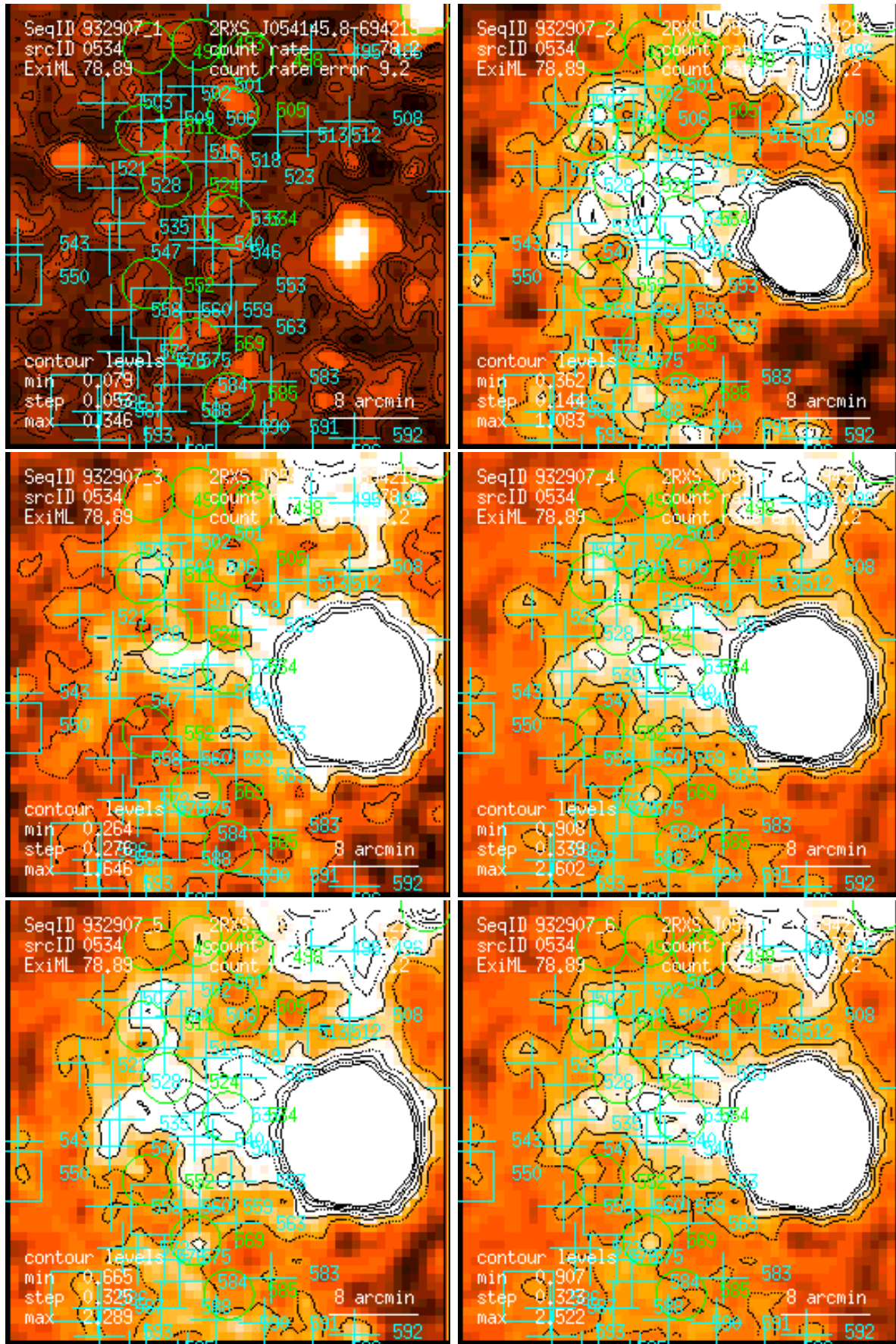
Figure 534: RASS 932907: detection 0534: band rate images, Gaussian filter: (1) PSPC channels 11 – 41, (2) 52 – 90, (3) 91 – 201, (4) 11 – 235, (5) 52 – 201, (6) 11 – 201. Broad band rates in counts/ks. Band rate contour levels in counts/ks/arcmin 2 .
