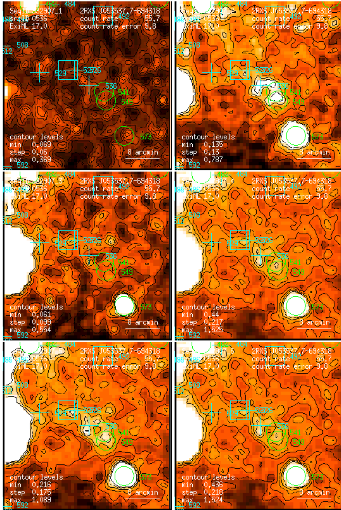
Figure 536: RASS 932907: detection 0536: band rate images, Gaussian filter: (1) PSPC channels 11 – 41, (2) 52 – 90, (3) 91 – 201, (4) 11 – 235, (5) 52 – 201, (6) 11 – 201. Broad band rates in counts/ks. Band rate contour levels in counts/ks/arcmin 2 .
