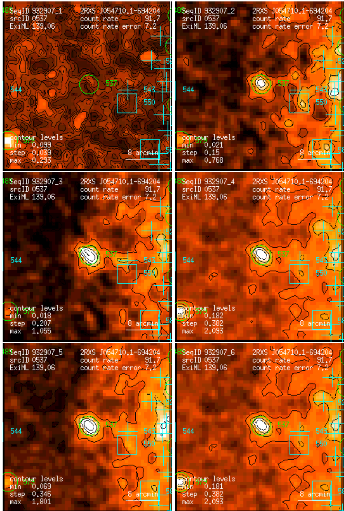
Figure 537: RASS 932907: detection 0537: band rate images, Gaussian filter: (1) PSPC channels 11 – 41, (2) 52 – 90, (3) 91 – 201, (4) 11 – 235, (5) 52 – 201, (6) 11 – 201. Broad band rates in counts/ks. Band rate contour levels in counts/ks/arcmin 2 .
