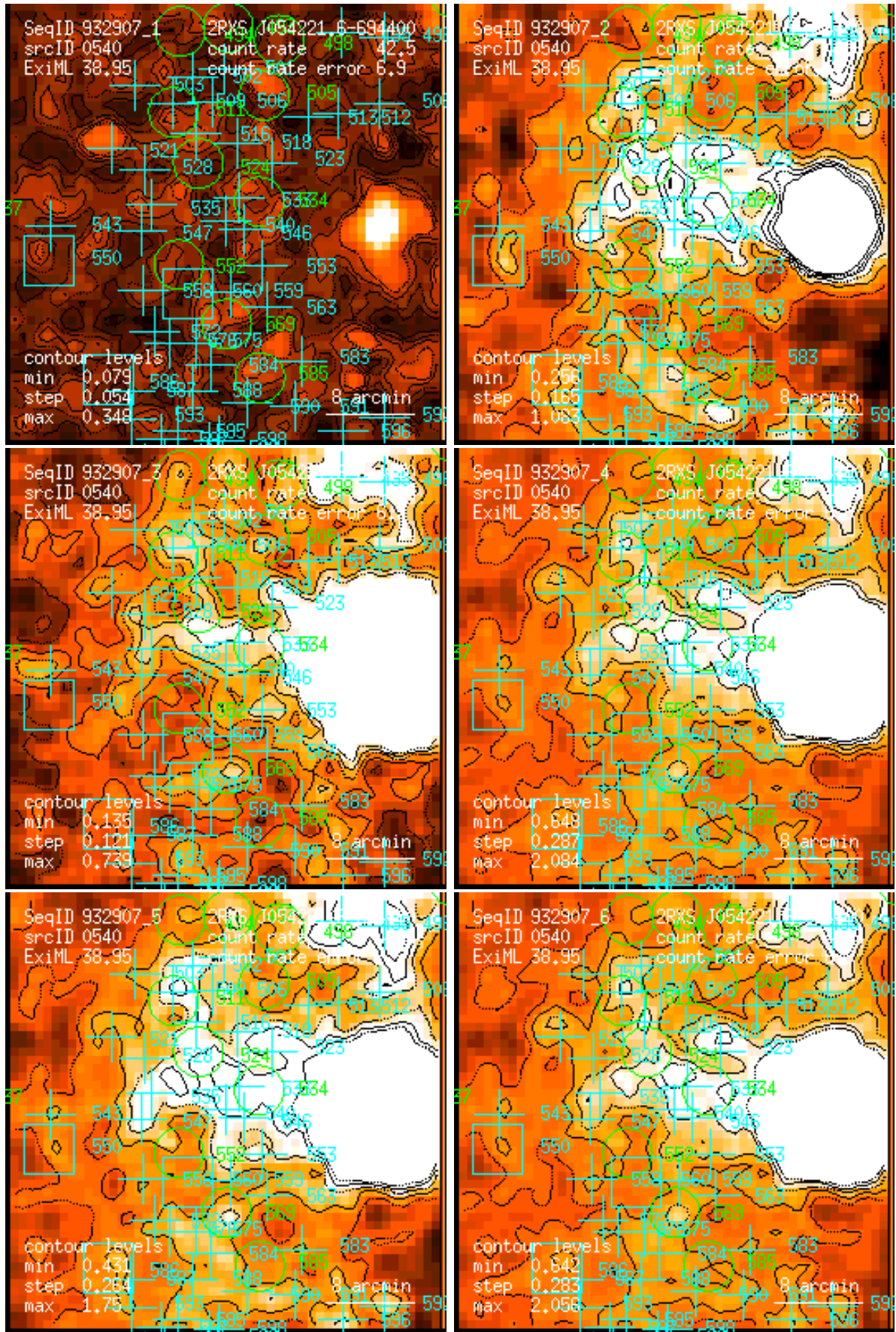
Figure 540: RASS 932907: detection 0540: band rate images, Gaussian filter: (1) PSPPC channels 11 – 41, (2) 52 – 90, (3) 91 – 201, (4) 11 – 235, (5) 52 – 201, (6) 11 – 201. Broad band rates in counts/ks. Band rate contour levels in counts/ks/arcmin 2 .
