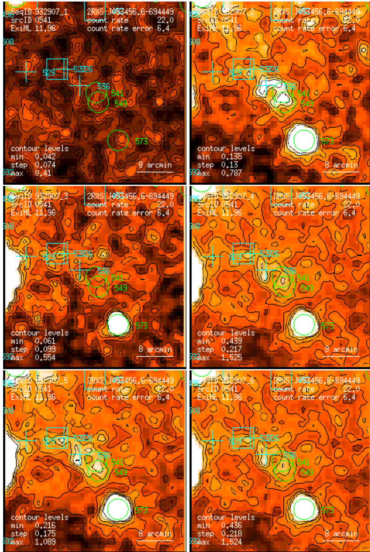
Figure 541: RASS 932907: detection 0541: band rate images, Gaussian filter: (1) PSPC channels 11 – 41, (2) 52 – 90, (3) 91 – 201, (4) 11 – 235, (5) 52 – 201, (6) 11 – 201. Broad band rates in counts/ks. Band rate contour levels in counts/ks/arcmin 2 .
