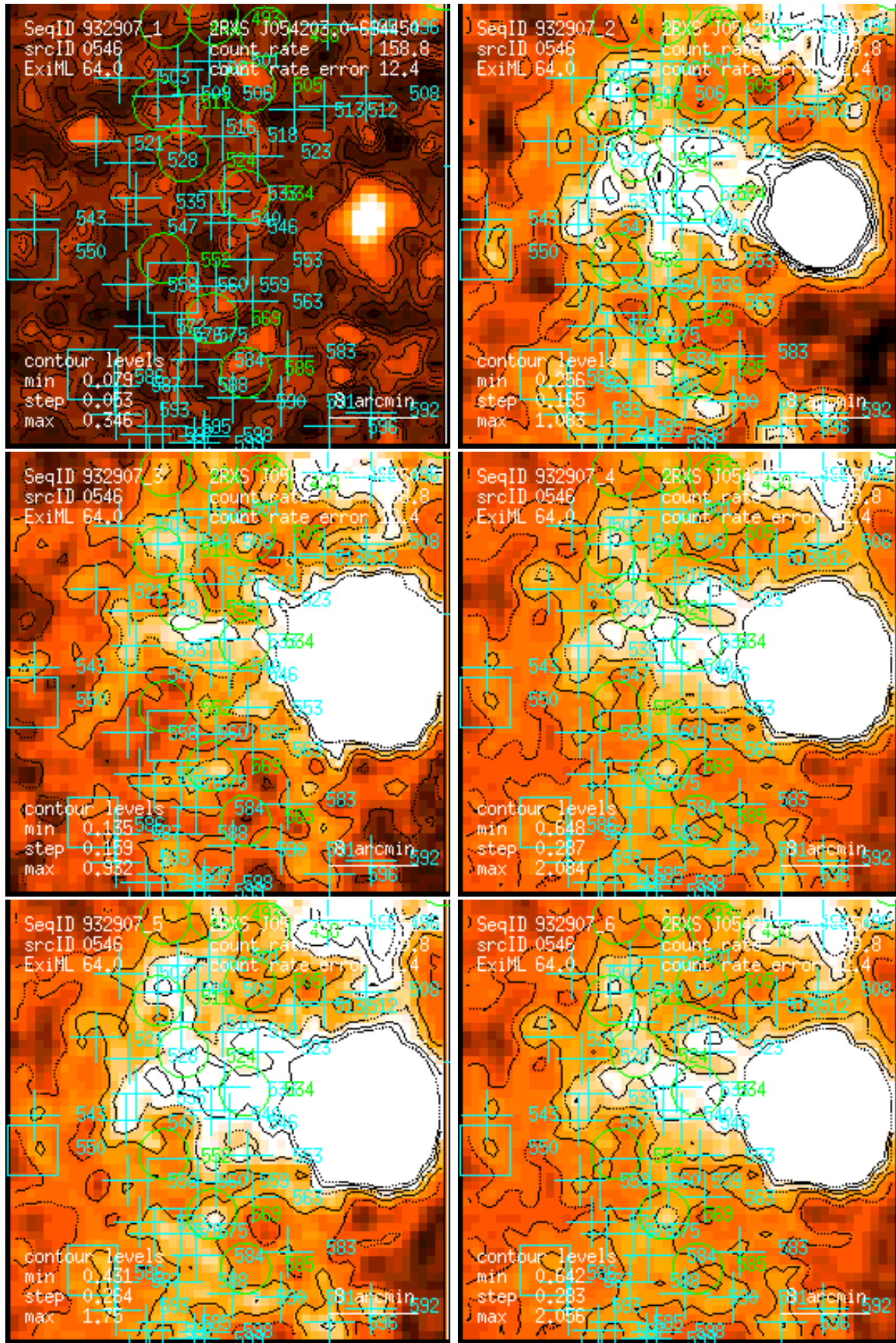
Figure 546: RASS 932907: detection 0546: band rate images, Gaussian filter: (1) PSPC channels 11 – 41, (2) 52 – 90, (3) 91 – 201, (4) 11 – 235, (5) 52 – 201, (6) 11 – 201. Broad band rates in counts/ks. Band rate contour levels in counts/ks/arcmin 2 .
