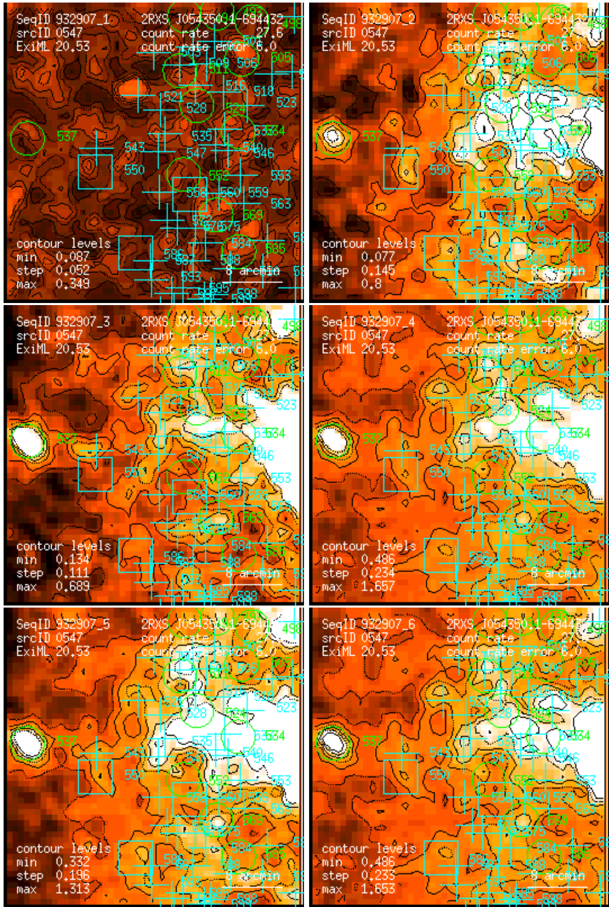
Figure 547: RASS 932907: detection 0547: band rate images, Gaussian filter: (1) PSPC channels 11 – 41, (2) 52 – 90, (3) 91 – 201, (4) 11 – 235, (5) 52 – 201, (6) 11 – 201. Broad band rates in counts/ks. Band rate contour levels in counts/ks/arcmin 2 .
