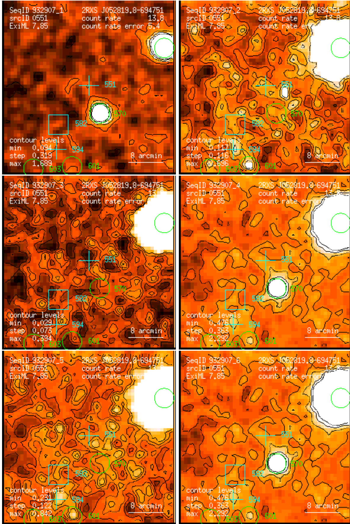
Figure 551: RASS 932907: detection 0551: band rate images, Gaussian filter: (1) PSPC channels 11 – 41, (2) 52 – 90, (3) 91 – 201, (4) 11 – 235, (5) 52 – 201, (6) 11 – 201. Broad band rates in counts/ks. Band rate contour levels in counts/ks/arcmin 2 .
